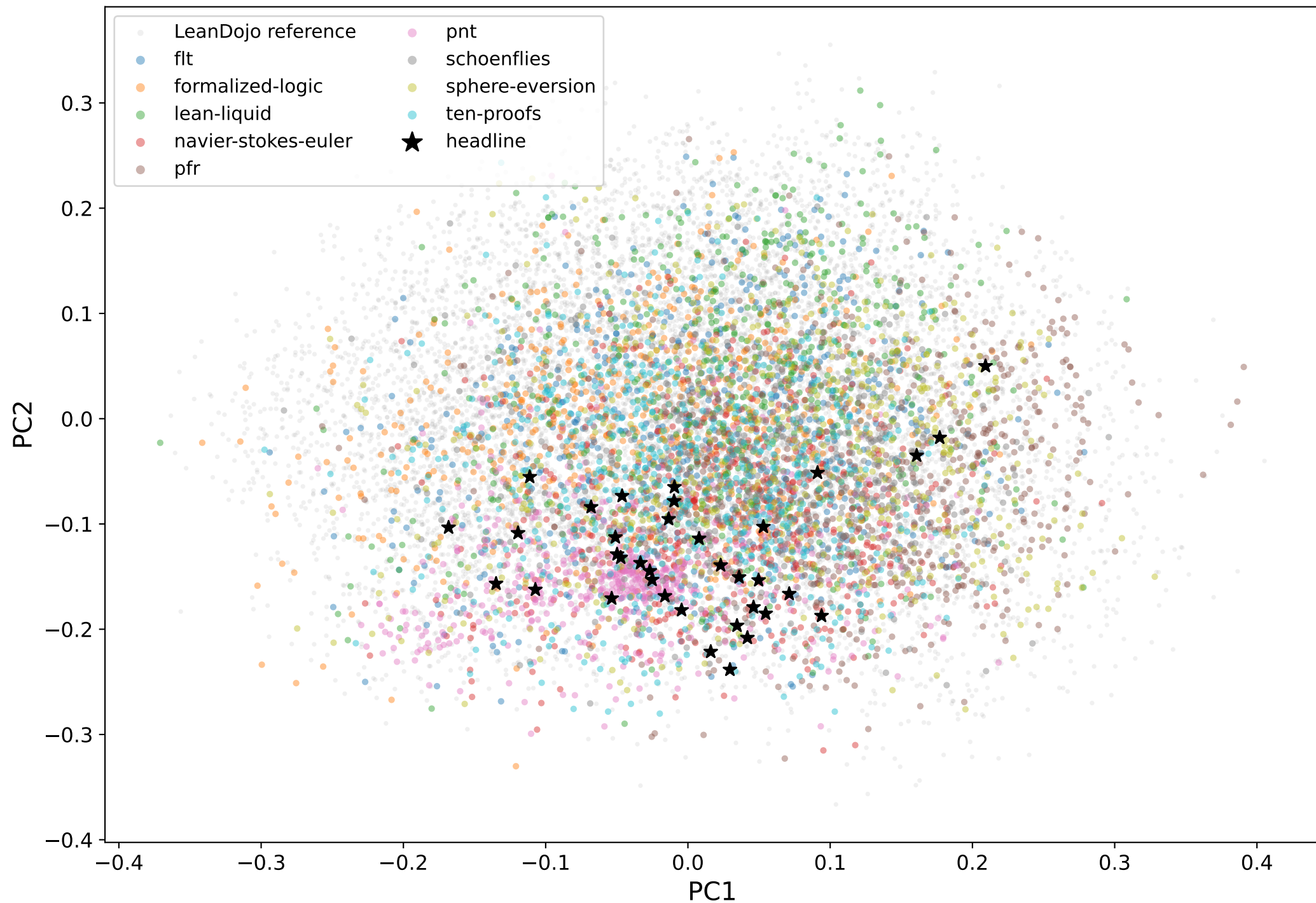
Frontier theorem statements in the frozen LeanDojo PCA space
