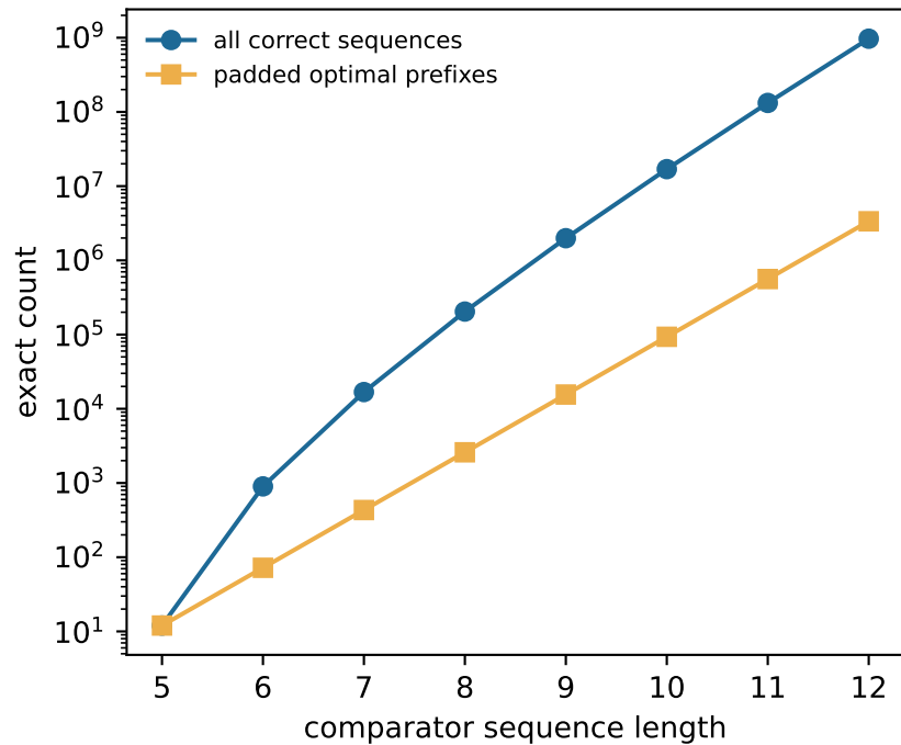
Correct but redundant forms proliferate
