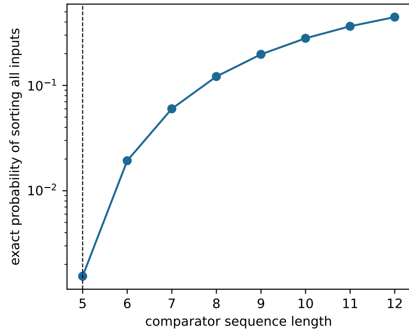
Correctness is rare at the boundary
