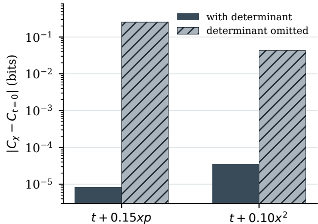
Gauge determinant removes false bits
