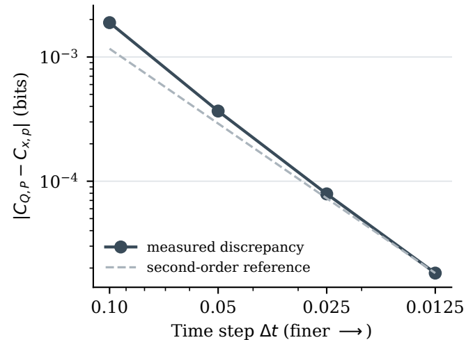
Canonical discrepancy vanishes
