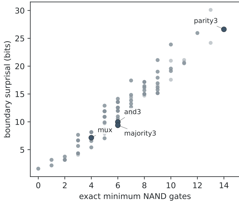
Minimal semantics can also be rare
