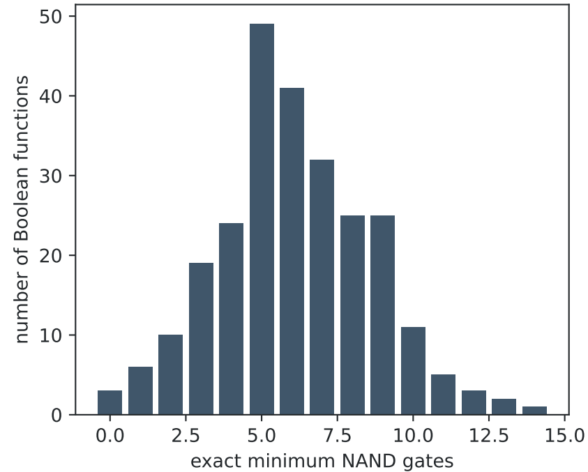
All 256 functions synthesized
