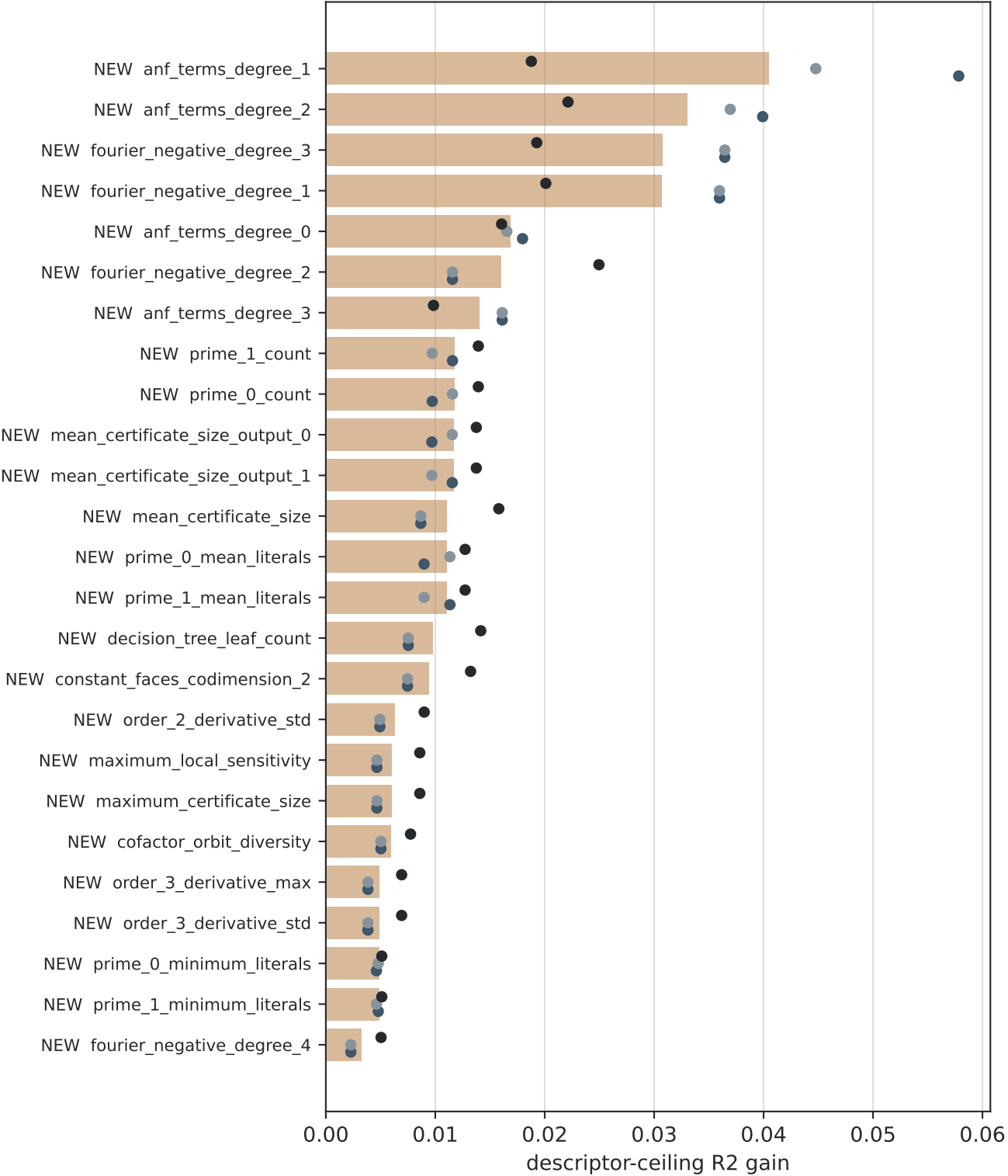
New information beyond original descriptor
