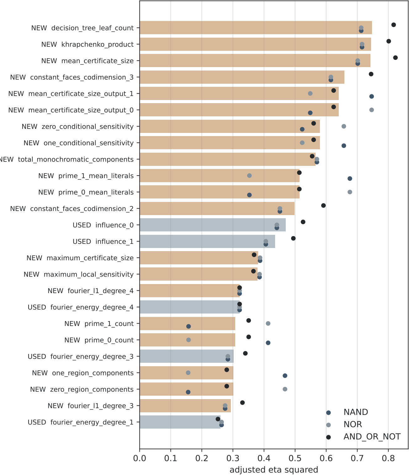
Standalone nonlinear association
