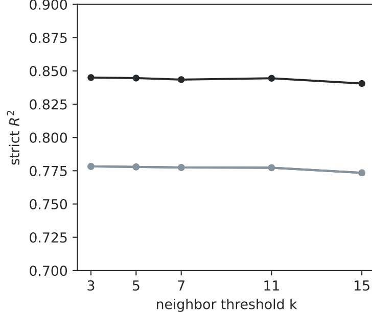
Neighbor sensitivity
