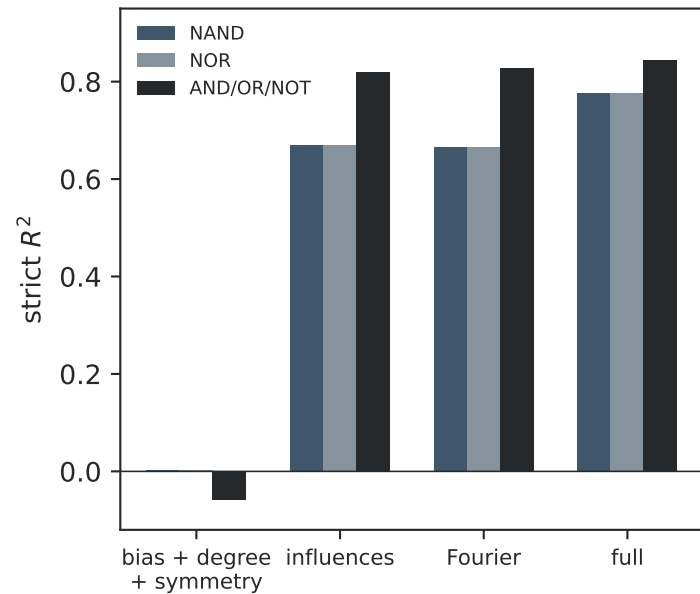
Feature ablations
