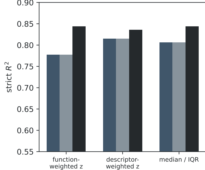
Scaling sensitivity
