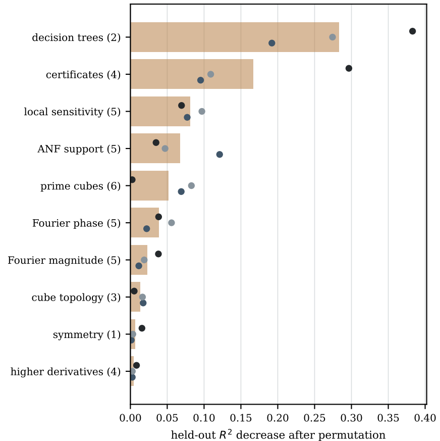
Joint feature families
