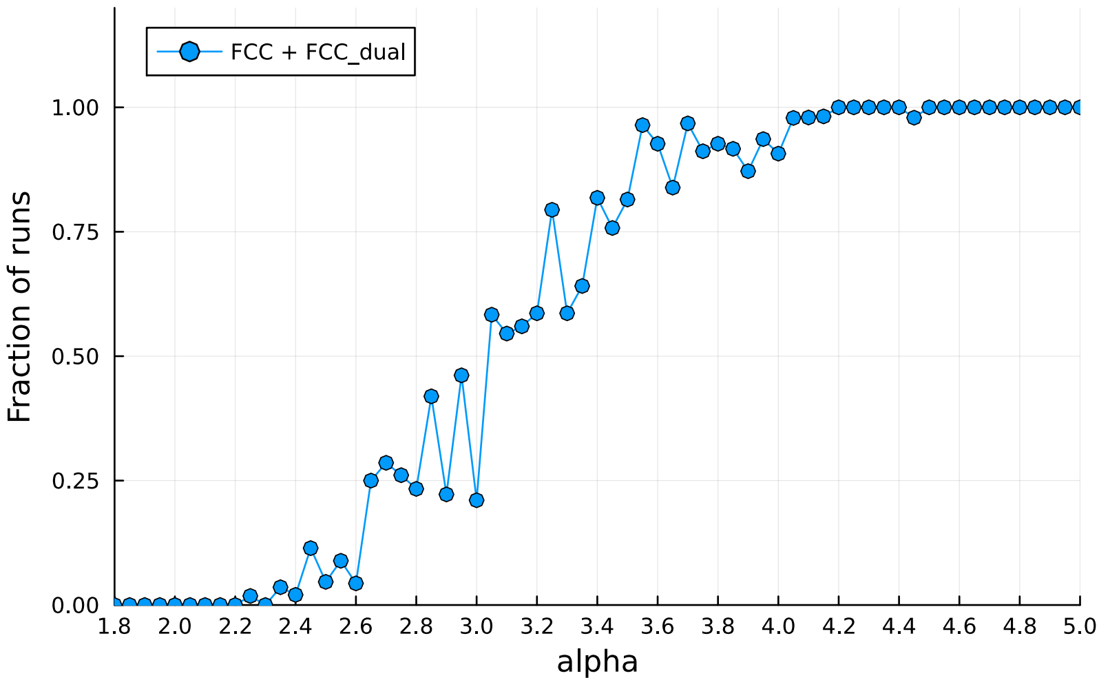
Fraction of runs converging to FCC-type minimizers
