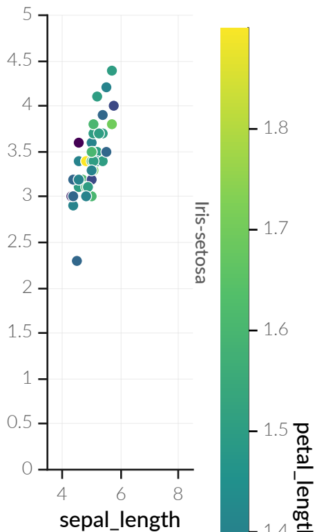
petal_width_bin
