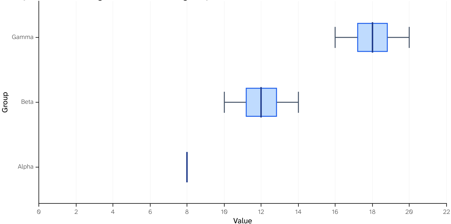
Box plot with a single-observation group
