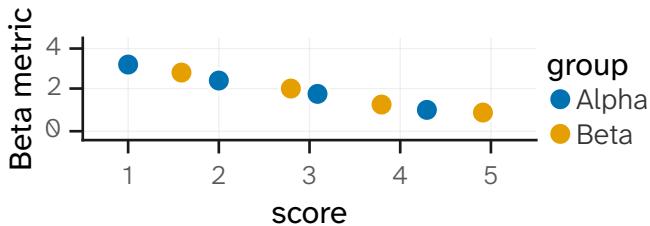
Beta metric
