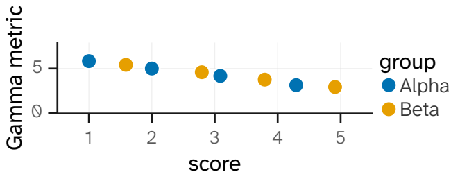
Gamma metric
