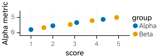
Alpha metric
