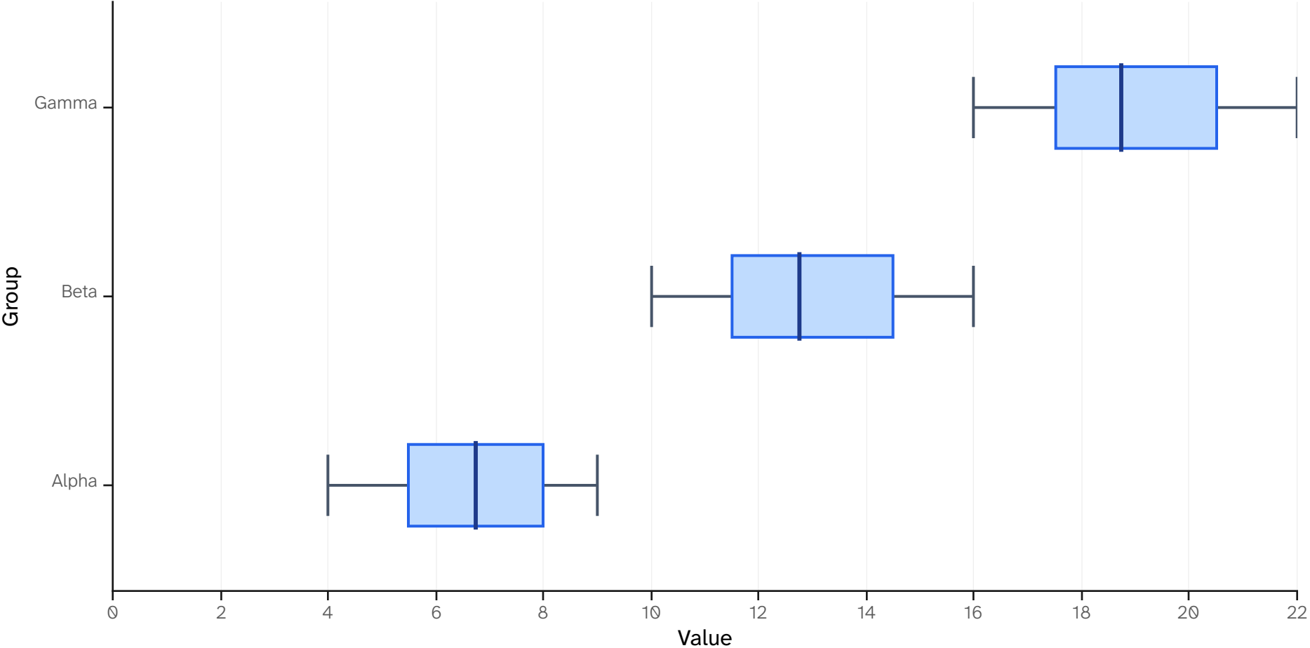
Box plot with no outliers
