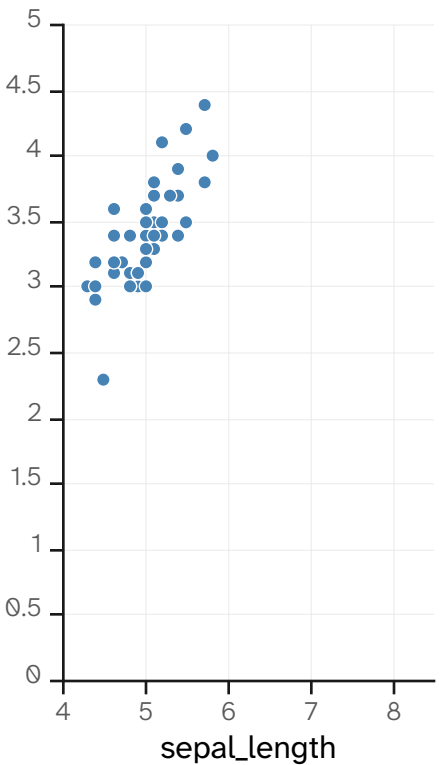
petal_width_bin
