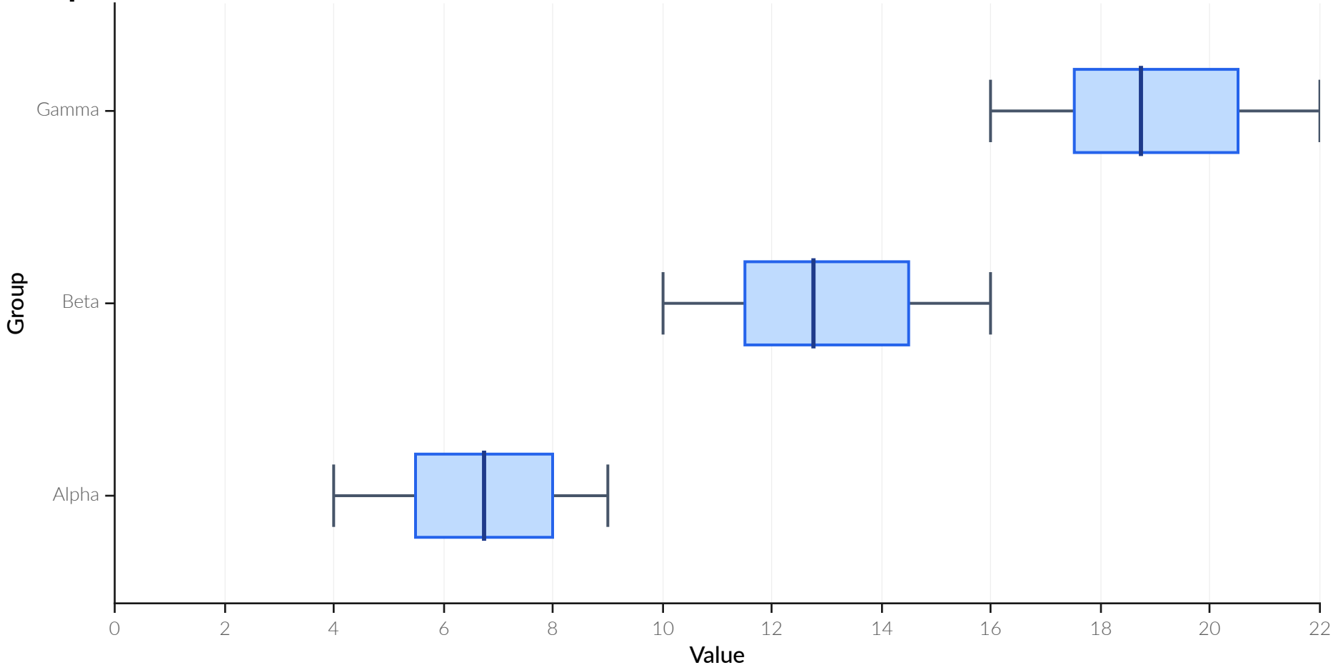
Box plot with no outliers
