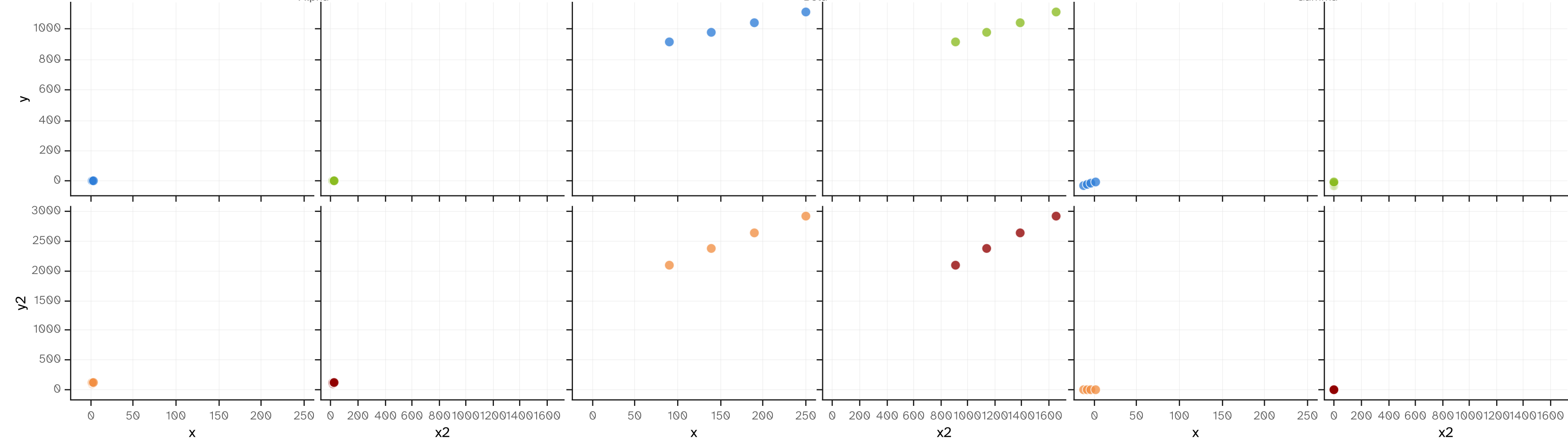
Alpha
