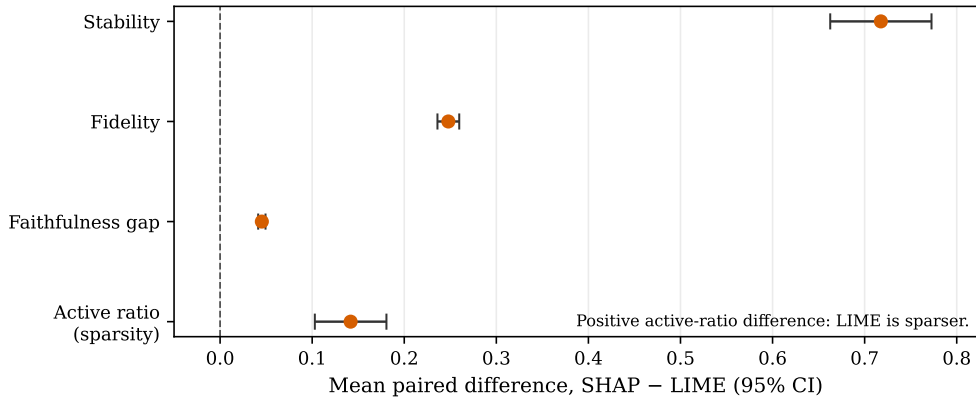
Figure 1: Mean paired difference (SHAP – LIME) with its 95% confidence interval for the quality-oriented primary endpoints ( n = 75 matched cells), as in Table 1. For the active ratio, a positive difference means SHAP is denser, that is, LIME is sparser
