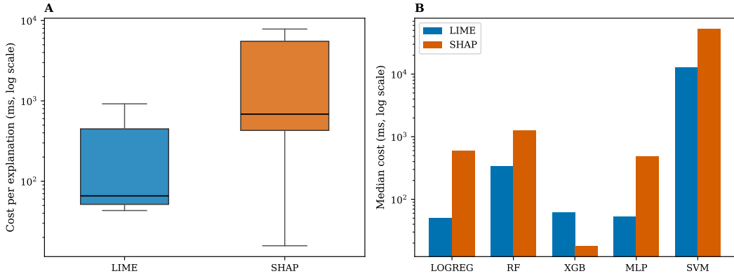
Figure 2: Runtime behavior under matched-cell pairing ( n = 75 ). (A) Overall cost distribution by method (log scale). (B) Model-level median cost (log scale), showing the XGBoost exception where SHAP is faster while other families are SHAP-slower
