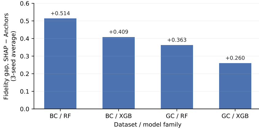
Figure 3: Cross-dataset extension: paired SHAP–Anchors fidelity gap (3-seed average) per dataset and model; the Anchors levels are in Table 4. BC = Breast Cancer; GC = German Credit
