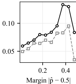
Anchors
