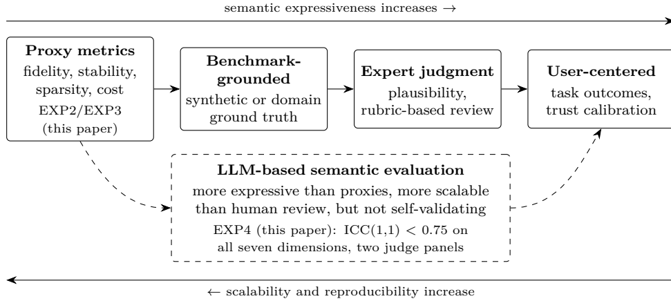
Figure 4: Evaluation continuum for post-hoc XAI, with representative metric families mapped to each evidence layer. LLM-based semantic evaluation occupies an intermediate position between proxy metrics and human review; the EXP4 reliability result (Section 4.4) shows it is not yet self-validating.
