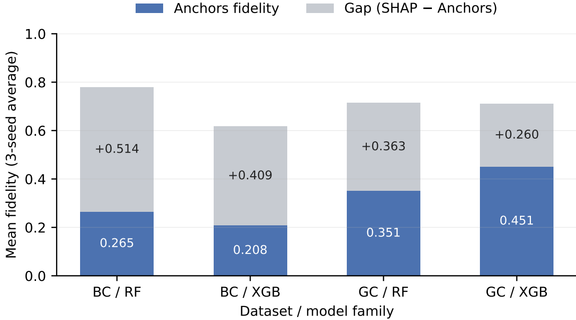
Figure 4: EXP3 external validation: mean Anchors fidelity (3-seed average, solid) with the paired SHAP–Anchors gap stacked above it (shaded), so each bar reaches the SHAP level without restating it. SHAP exceeds Anchors in all 12 paired (dataset \times model \times seed) combinations. BC=Breast Cancer; GC=German Credit.
