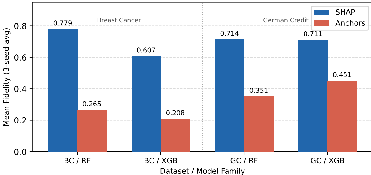
EXP3: SHAP vs. Anchors Fidelity Across Datasets (External Validation)
