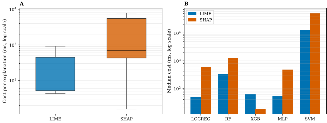
Figure 2: Runtime behavior under matched-cell pairing ( n = 75 ). (A) Overall cost distribution by method (log scale). (B) Model-level median cost (log scale), showing the XGBoost exception where SHAP is faster while other families are SHAP-slower
