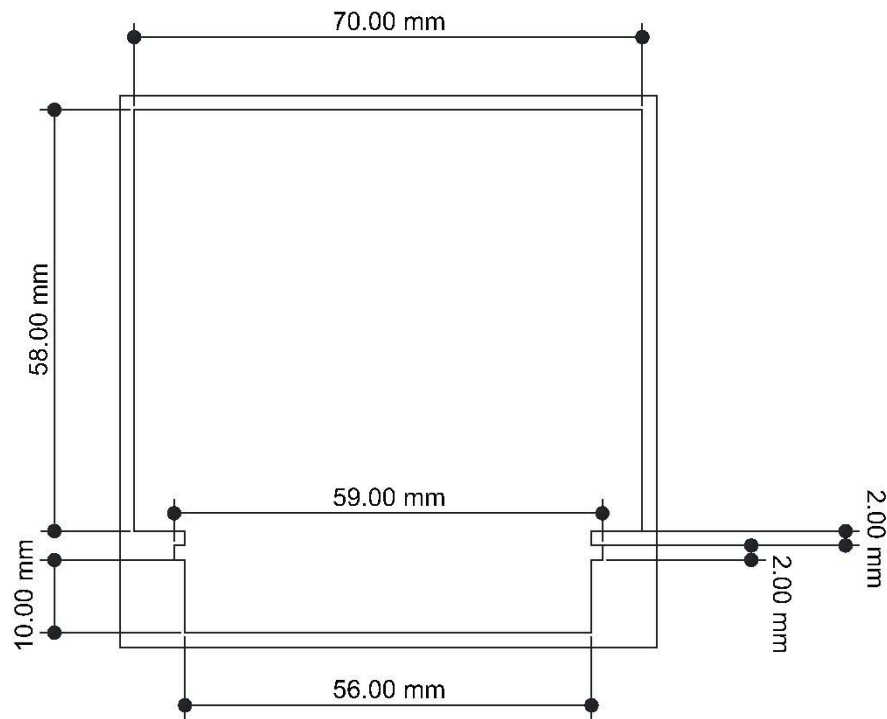
Cross Dimensions
