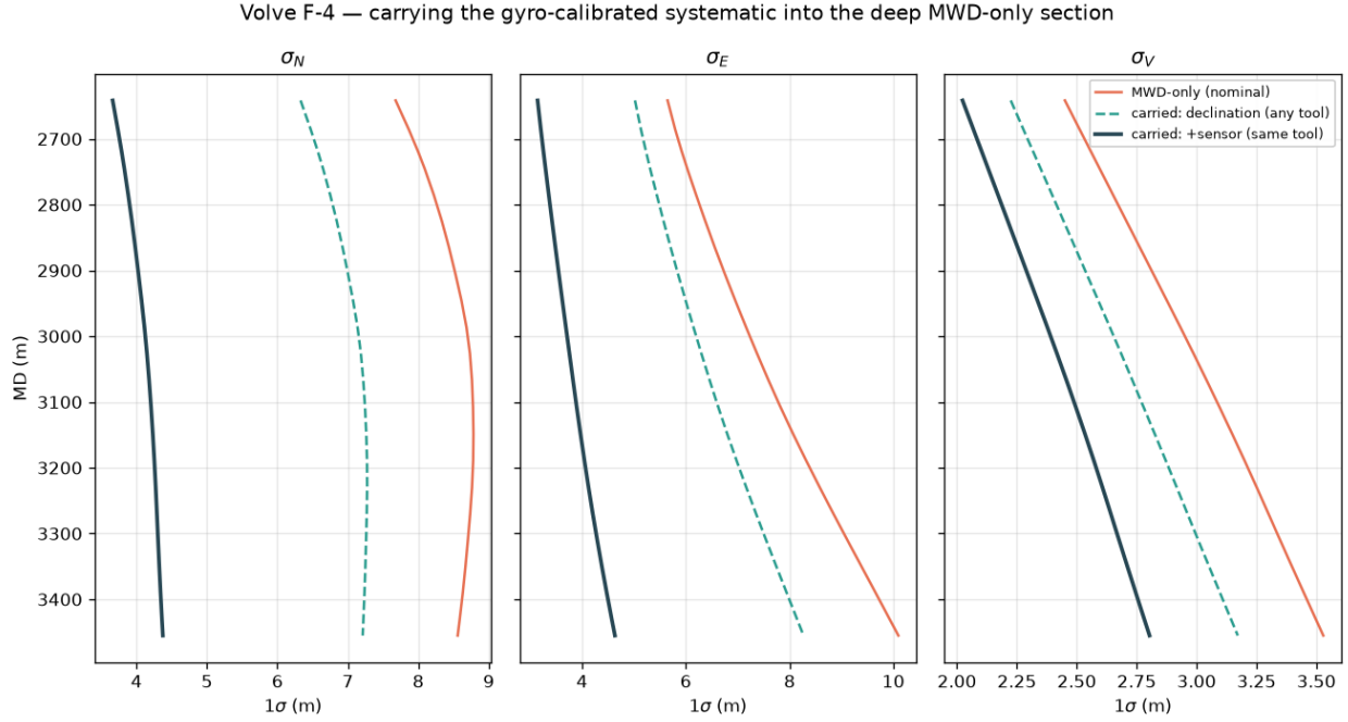
Figure 3: Figure 2. Carrying the gyro calibration into the deep MWD-only section on Volve F-4. Dashed: declination only (unconditional). Solid: plus sensor systematic (same MWD tool reused). Both stay below the nominal MWD-only covariance throughout.
