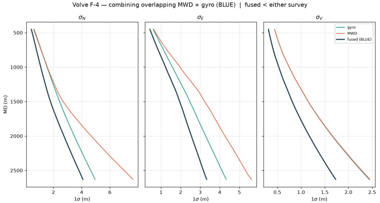
Figure 2: Figure 1. Combining overlapping MWD and gyro on Volve F-4 (BLUE). The fused curve is below either input on all three axes.
