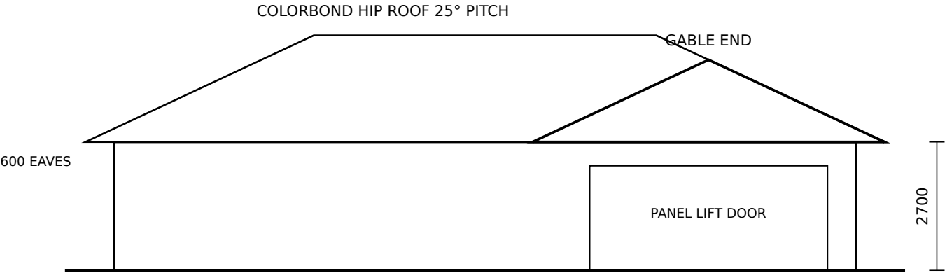
SOUTH ELEVATION (STREET)
