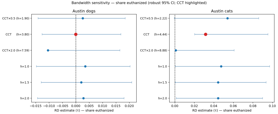
Figure 8: Bandwidth Sensitivity Euthanized
