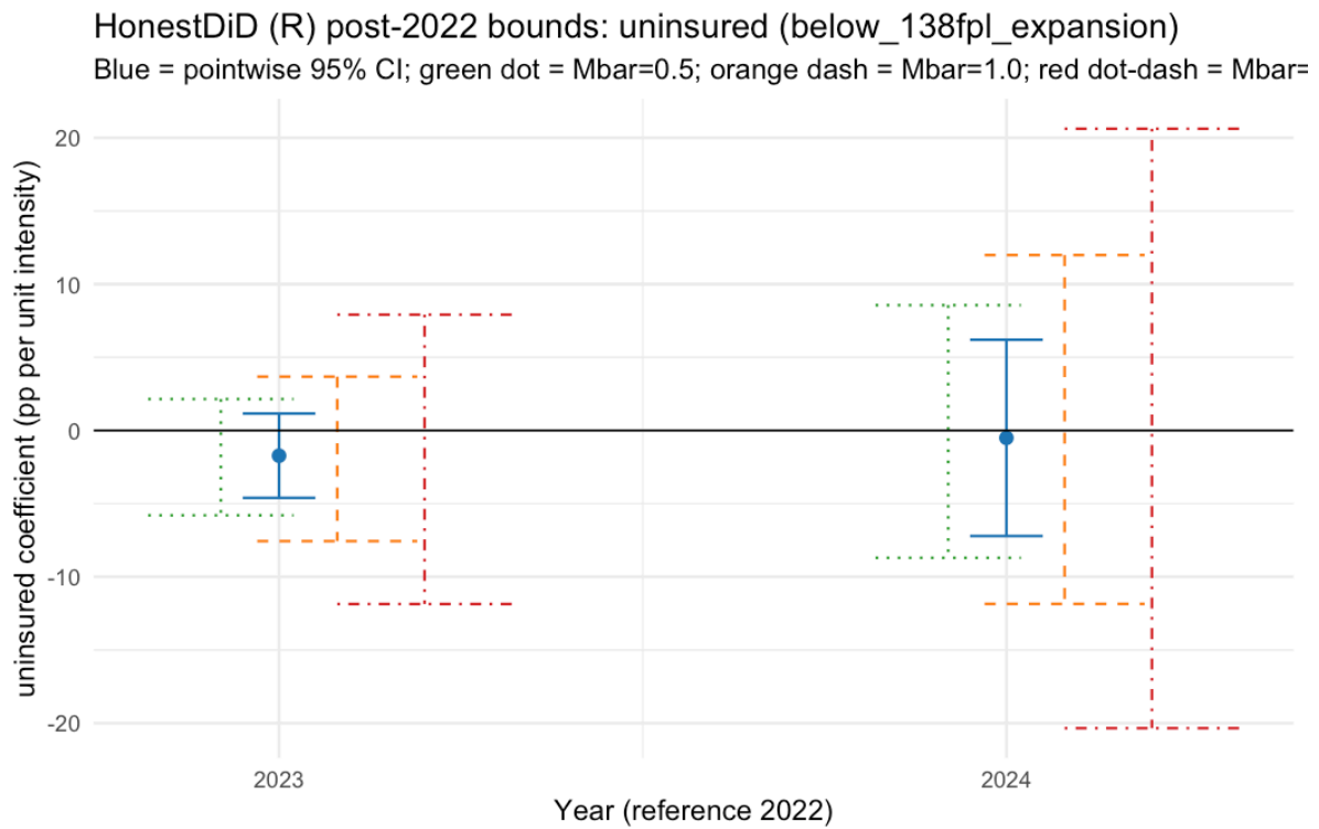
Figure 11: R Honestdid Uninsured Below 138Fpl Expansion
