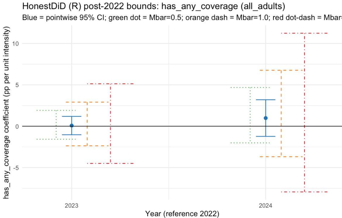
Figure 1: R Honestdid Has Any Coverage All Adults
