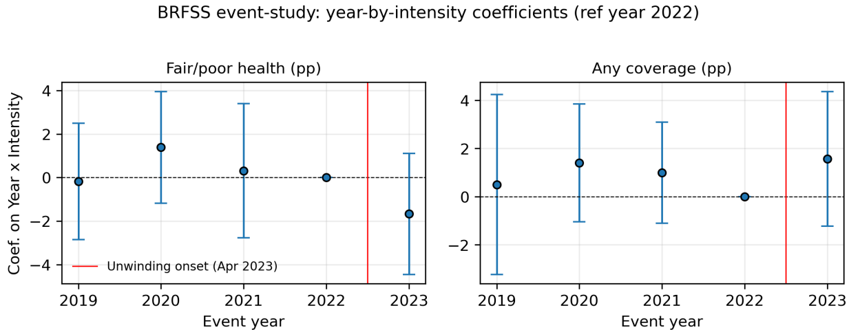
Figure 12: Brfss Event Study Main
