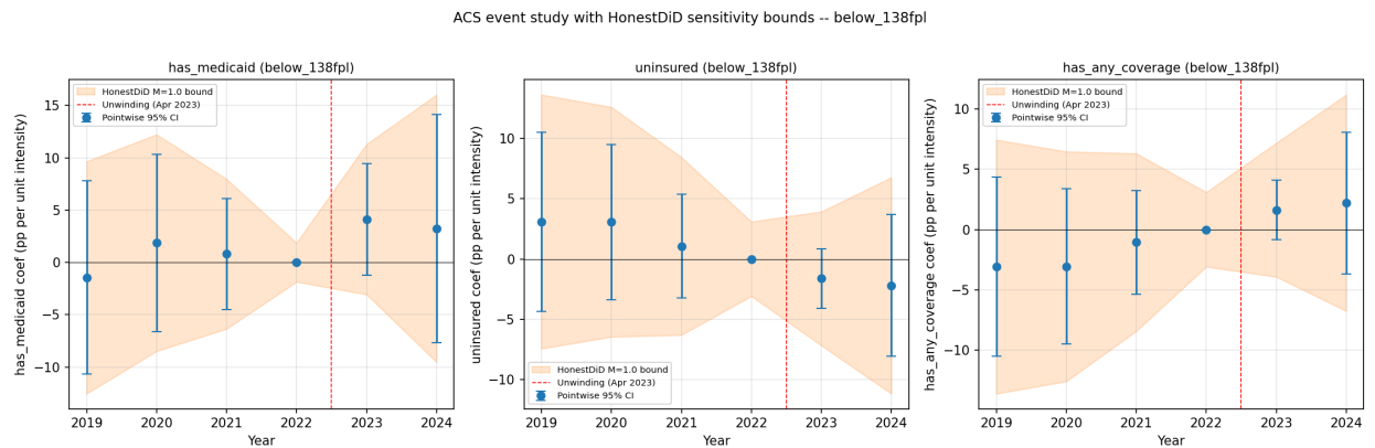
Figure 7b: ACS event study with HonestDiD bounds, below 138% FPL sample (all three coverage
