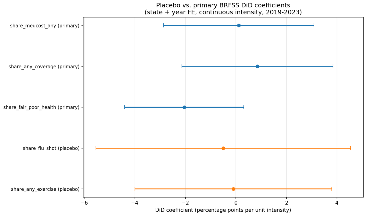
Figure 6: Placebo vs. primary BRFSS DiD coefficients on the same scale (continuous intensity,
