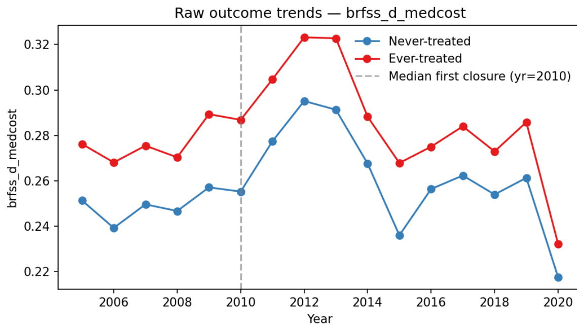
Figure 19: Fig1 Raw Trends Brfss D Medcost
