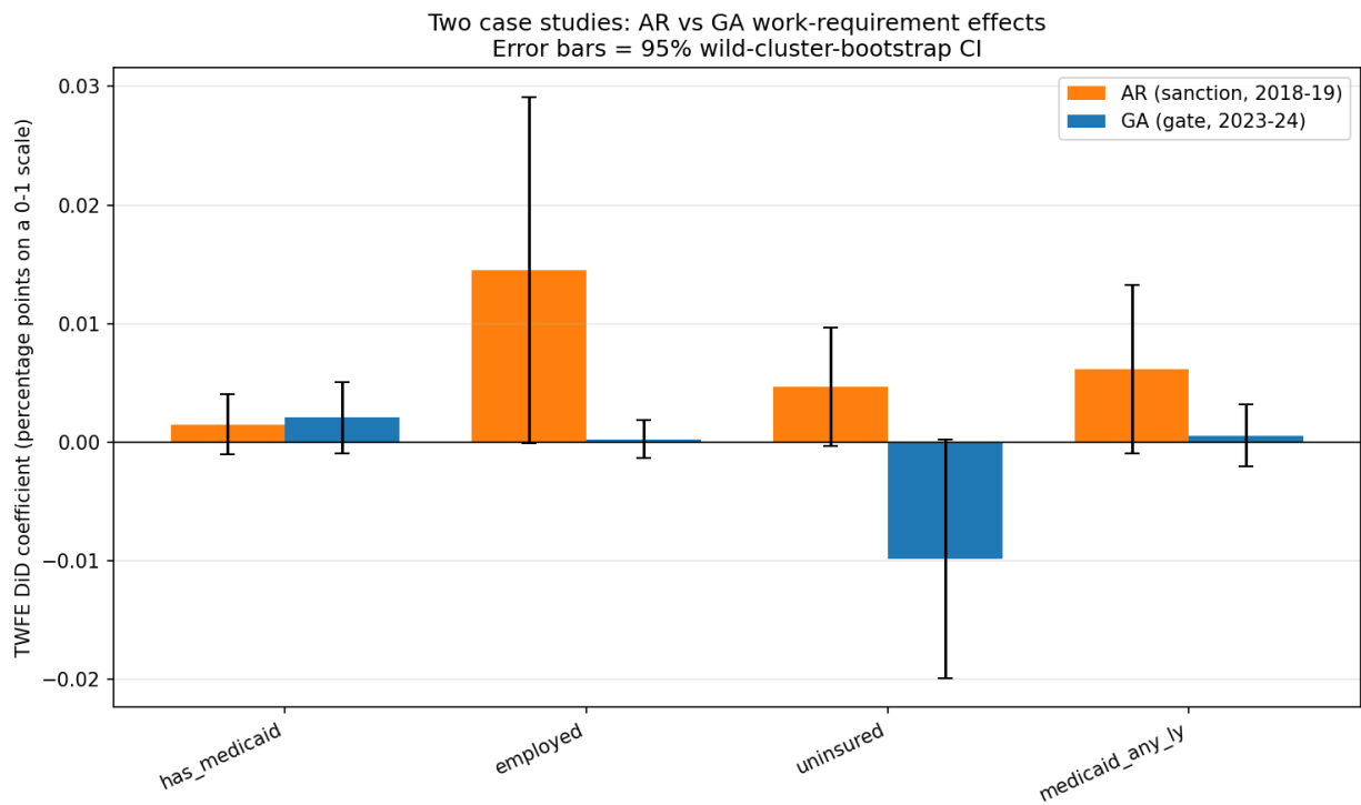
Figure 3: Side-by-side comparison bar chart of AR and GA coefficients with 95% wild bootstrap
