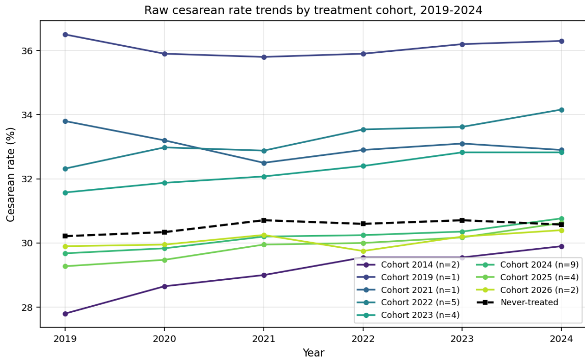
Figure 1: Raw cohort-specific cesarean trends
