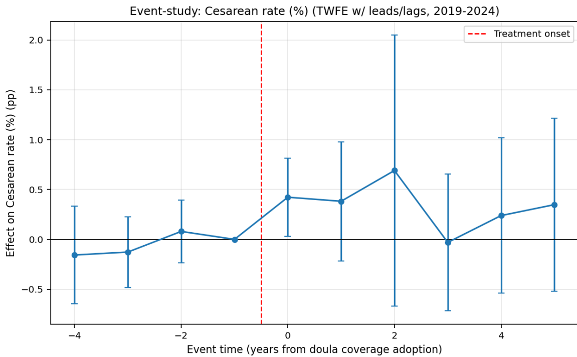
Figure 2: Main event-study with confidence bands
