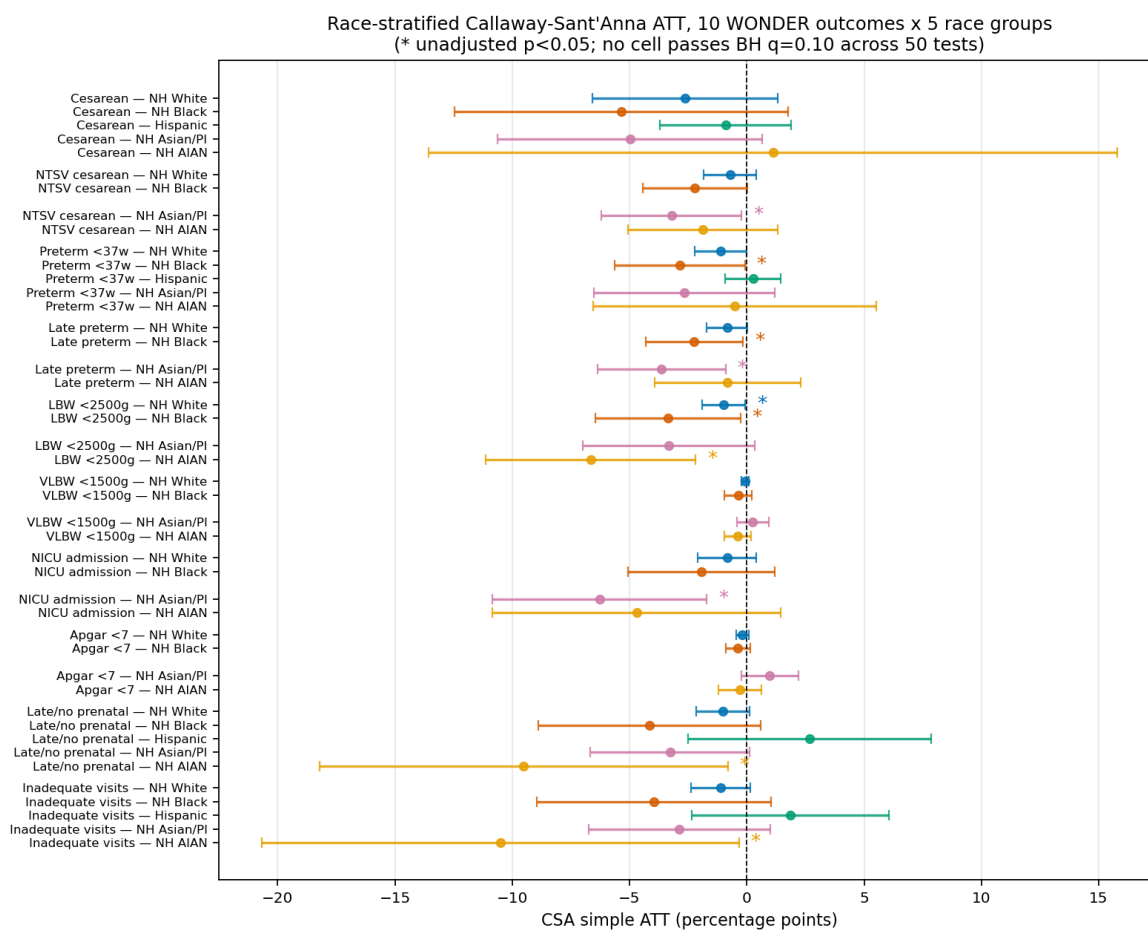
Figure 8: Full race-stratified forest plot
