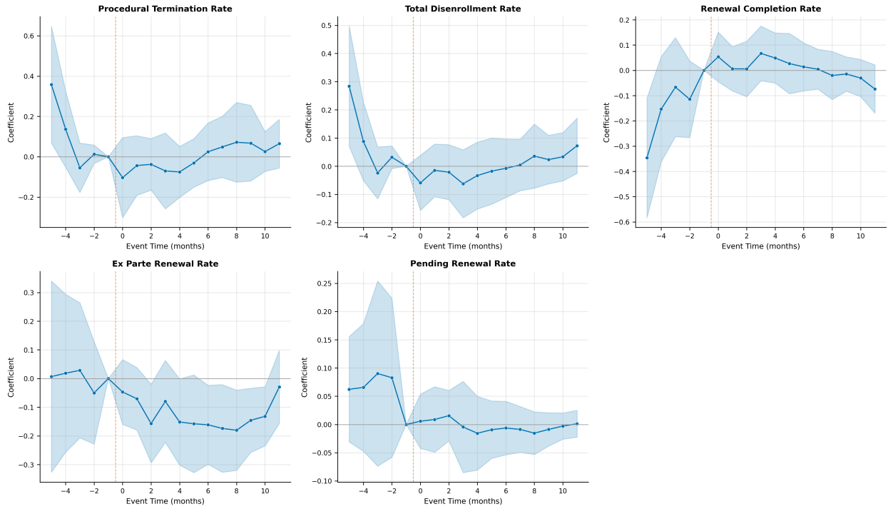
Figure 1: Fig3 Event Study Panel
