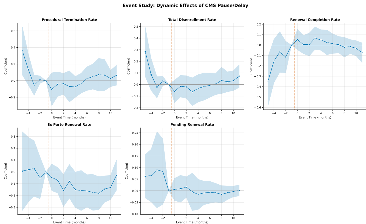
Figure 3: Fig3 Event Study Panel
