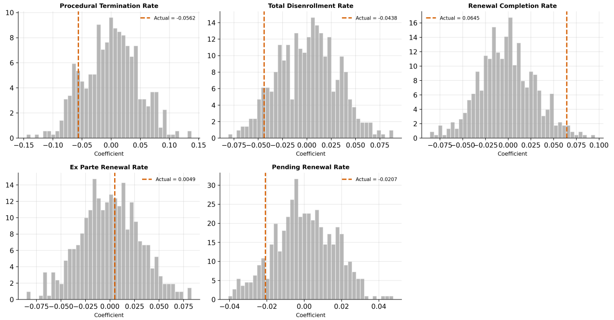
Figure 2: Fig4 Placebo Test
