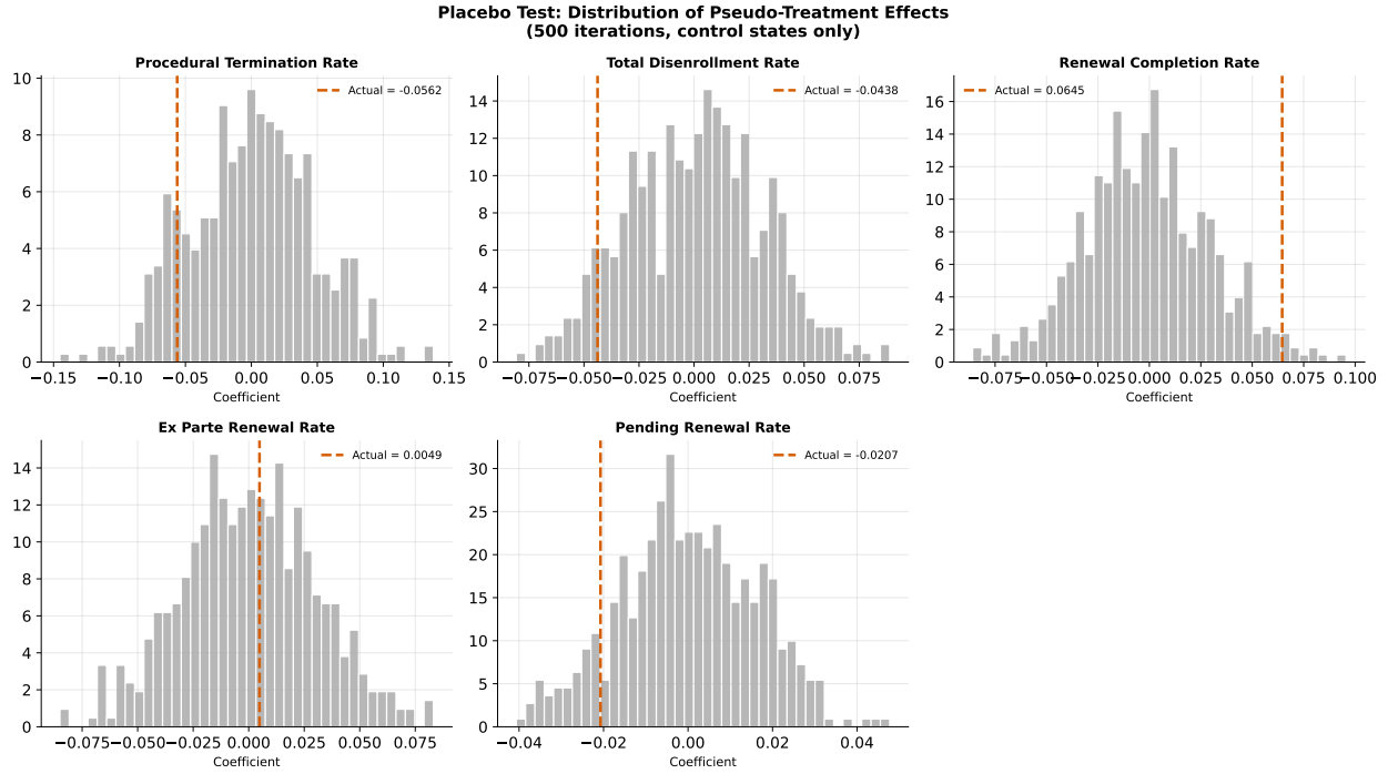
Figure 4: Fig4 Placebo Test
