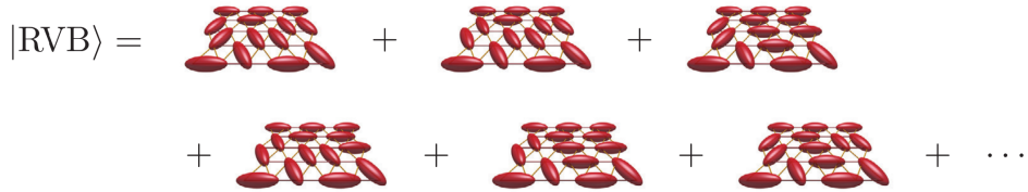
Figure 5: Anderson's resonating valence bond (RVB) state, where the ellipsoids represent the possible spin singlet pairings [5](p.2).
