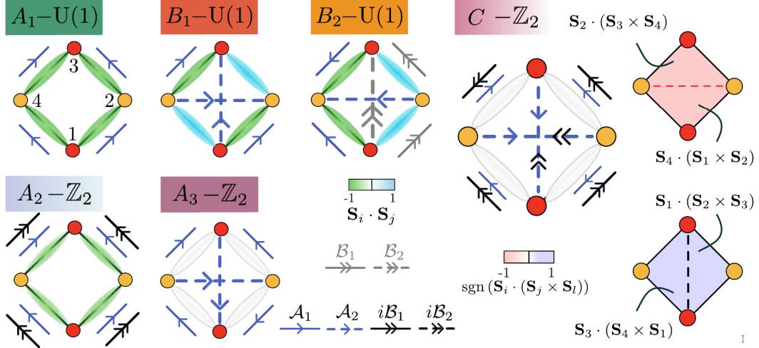
Figure 6: Schwinger boson Ansatzes associated with the six magnetic phases of Table 1. Blue arrows denote real singlet amplitudes A_{ij} , black and gray arrows denote real and imaginary hopping amplitudes B_{ij} . The colored ellipses show the correlators \langle \mathbf{S}^{\text{EP}} \rangle evaluated in the gapped spin-liquid regime. For the Ansatz of phase C the staggered chirality pattern \langle \chi^{\text{EP}} \rangle is nonzero as well. Adapted from Ref. [1].
