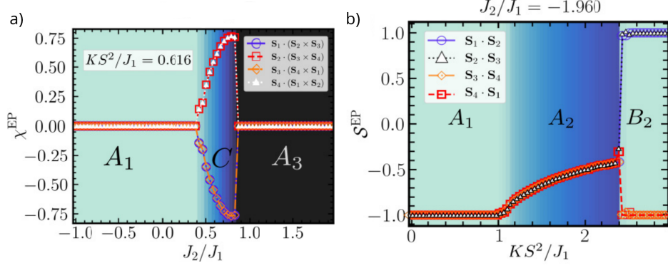
Figure 4: Scalar spin chiralities \chi^{\text{EP}} (a) and nearest-neighbor spin products \mathcal{S}^{\text{EP}} (b) along one-dimensional cuts through the phase diagram. The chirality grows continuously at the second-order transition from A_1 to C , this order holds as well for the transition from A_1 to A_2 . Adapted from Ref. [1].
