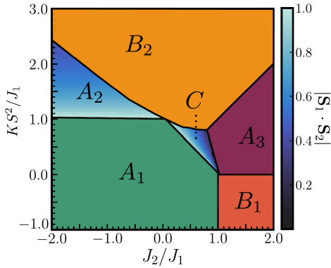
Figure 2: Classical phase diagram of the model in the (J_2, K) plane, obtained by minimizing the energy of the Ansatz (2).
