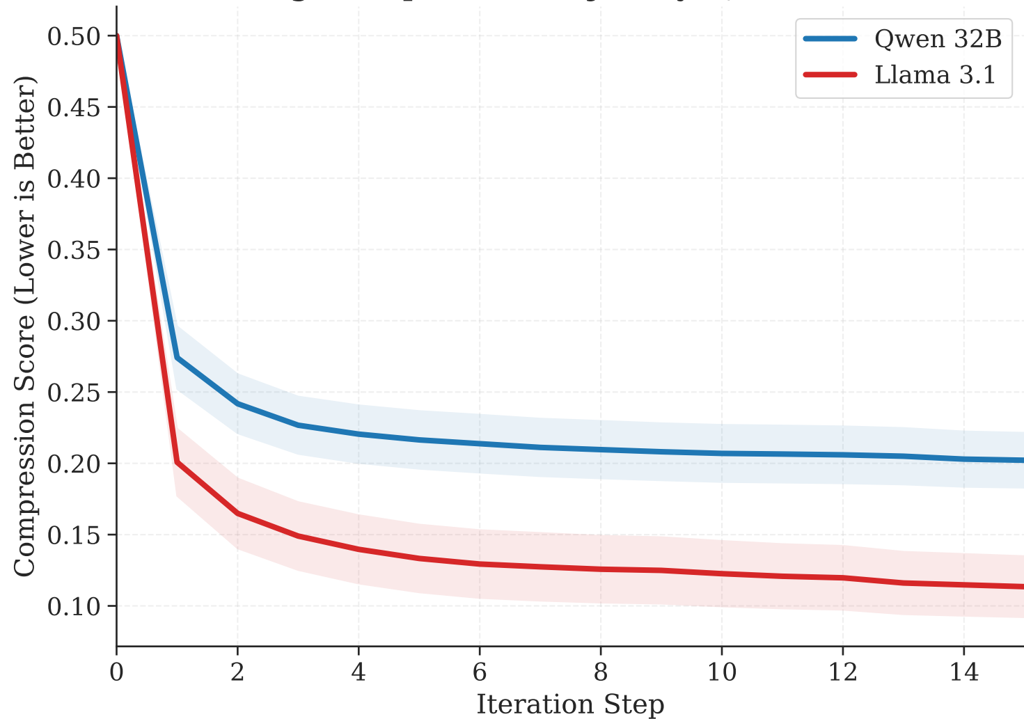
Average Compression Trajectory: Qwen vs Llama
