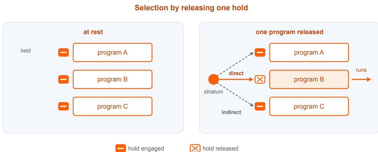
Figure 6.10 — Action selection by disinhibition. At rest, the output cells of the basal ganglia fire steadily and hold every motor program back. The direct pathway silences the cells holding back one program, which releases it. The indirect pathway strengthens the hold on the competing programs.
