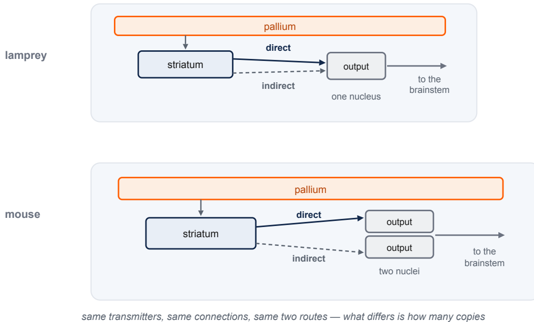
Figure 6.12 — The same selection circuit in a lamprey brain and a mouse brain, drawn as two matching circuit diagrams. The input stage, the output cells, and the direct and indirect routes between them are present in both, with the same transmitters. In the mammal the output nucleus is divided in two.
