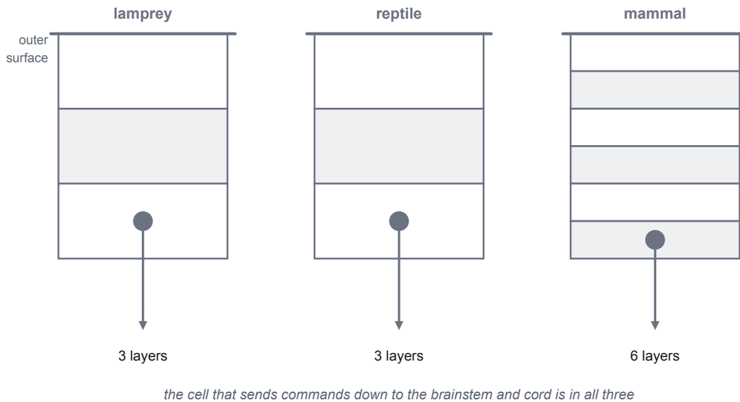
Figure 6.13 — The pallium in three vertebrates. A lamprey has three layers, a reptile has three, and a mammal has the six layers of the neocortex. The output cells that project down to the brainstem and spinal cord are present in all three.
