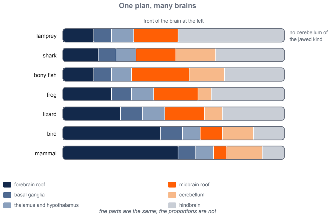
Figure 6.14 — One plan, many brains. Lamprey, shark, bony fish, frog, lizard, bird and mammal brains, each drawn as a bar of the same length and divided among the homologous regions in matching colors. The parts are the same and the proportions are not. The lamprey lacks a cerebellum of the kind jawed vertebrates have.
