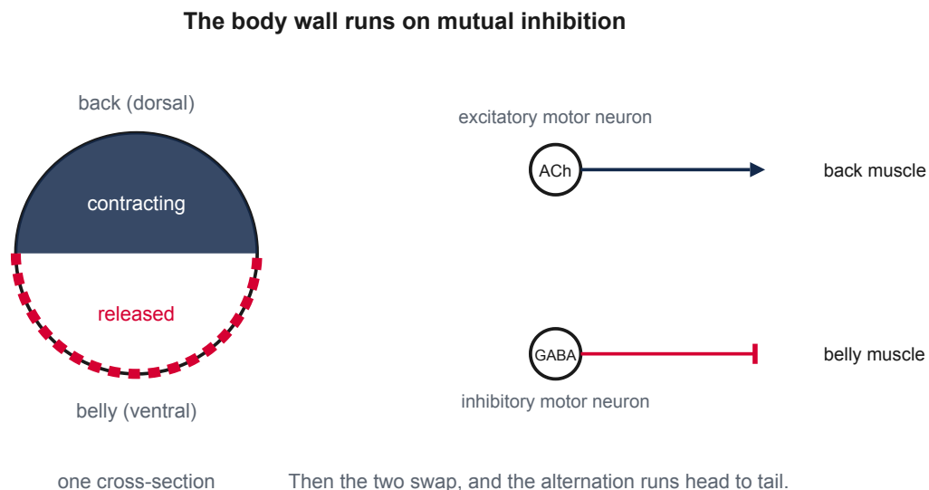
Figure 4.14 — The worm in cross-section, with the muscle on one side contracting while the muscle on the other is released, and the two motor neurons that hold that arrangement. The excitatory neuron releases acetylcholine onto the contracting side; the inhibitory neuron releases GABA onto the released side. The sides are the animal's back and belly, not its left and right.
