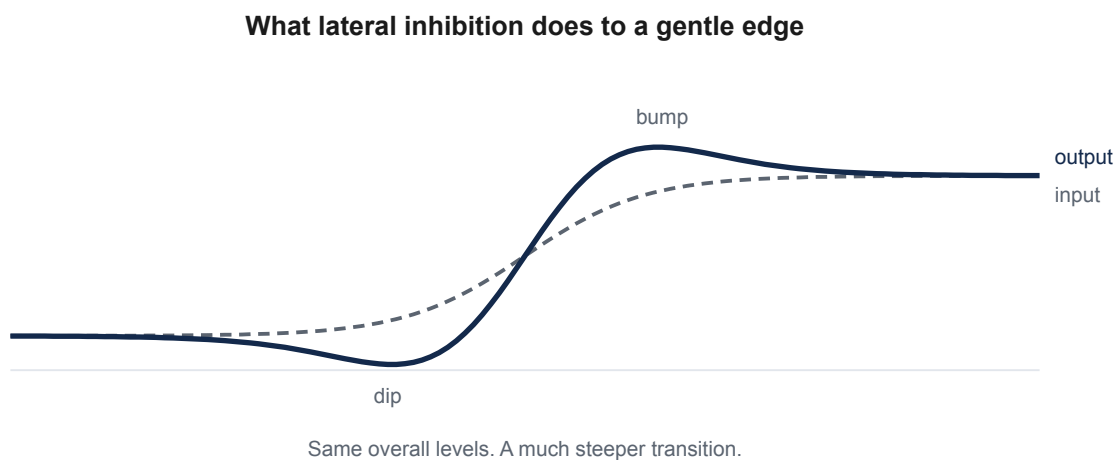
Figure 4.9 — What lateral inhibition does to a gentle edge. The input rises gradually from a dark region to a light one. The output, drawn over it, has the same overall levels but a much steeper transition, with a dip on the dark side of the edge and a bump on the light side.
