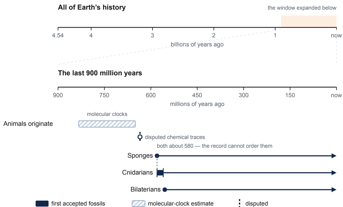
Figure 4.1 — The stretch of time this chapter's story runs through, drawn twice. The upper strip is all of Earth's history; the shaded window at its right-hand end is expanded below. Sponges, cnidarians and bilaterians each begin at their oldest widely accepted fossils and continue as lines to the present, because all three groups are still here. Two of the marks are ranges rather than dates: the origin of animals, because it comes from molecular clocks rather than from fossils, and the first cnidarians, because the identifications are argued about.
