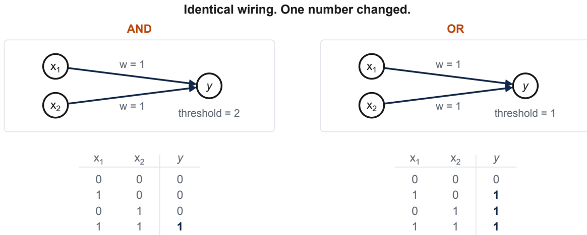
Figure 4.7 — Two units with identical wiring and different numbers. Each receives the same two excitatory inputs, each of weight one. The unit on the left has a threshold of two and fires only when both inputs arrive. The unit on the right has a threshold of one and fires when either does. The truth table beneath each shows what it produces for all four combinations.
