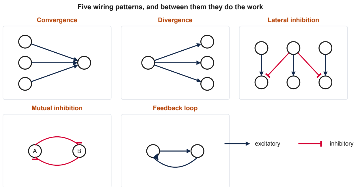
Figure 4.5 — The five circuit motifs used in this section, drawn in one panel. Convergence and divergence are the two simplest. Lateral inhibition sharpens a difference, mutual inhibition forces a choice, and a feedback loop keeps activity running after its input has stopped. Each is returned to, one at a time, in the subsections that follow.
