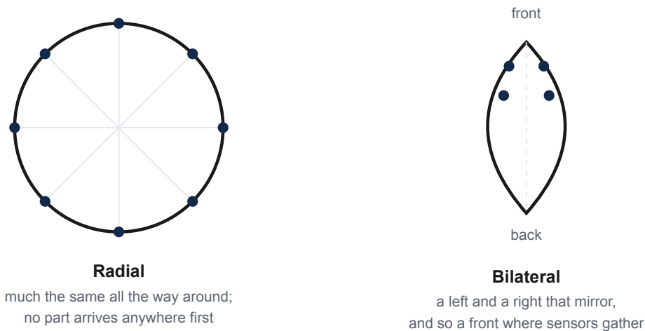
Figure 4.3 — Two body plans, drawn from above. The radial body is built around a central axis and is much the same in every direction, so no part of it arrives anywhere first and sensors have no privileged place to gather. The bilateral body has a left and a right that mirror each other and, consequentially, a front and a back, with the sensors and the neurons they report to gathered at the end that arrives first.
