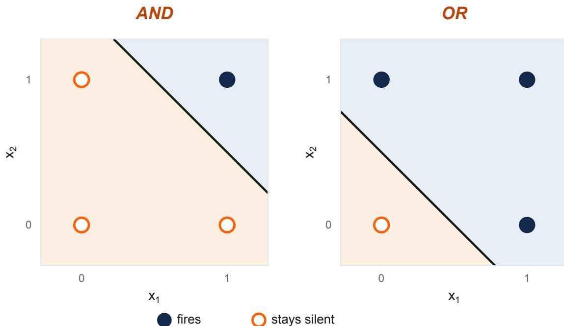
Figure 4.8 — The same four inputs, plotted twice. Each point is one combination of x_1 and x_2 : blue where the circuit should fire, orange where it should not. The shaded background shows what a circuit with that decision boundary actually does, so a correct circuit is one whose shading matches its points. For AND only (1,1) is blue; for OR only (0,0) is orange. The two boundaries are parallel, because going from one to the other shifts the line without rotating it.
