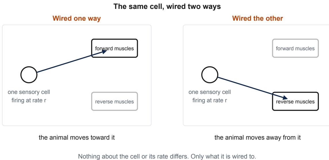
Figure 4.11 — One sensory cell, drawn twice, with everything about the cell held the same. On the left its output is routed to the muscles that drive the animal forward, and whatever it responds to becomes something the animal approaches. On the right the identical cell, firing at the identical rate, is routed to the muscles that drive a withdrawal, and the same thing becomes something the animal avoids.
