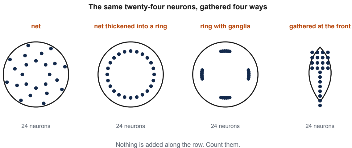
Figure 4.12 — The same nervous system at four degrees of concentration: a net spread evenly through the body wall, a net thickened into a ring, a ring with distinct clusters of cell bodies, and a bilateral body with its largest clusters gathered at the leading end. Nothing is added along the row. Neurons are only gathered into fewer places.
