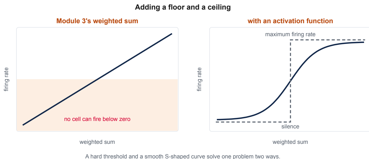
Figure 4.6 — Module 3's weighted sum, before and after an activation function is added. On the left the bare sum runs off the bottom of the plot into firing rates no cell can produce. On the right the same sum is squashed into the range between silence and the cell's maximum rate, by a hard threshold and by a smooth S-shaped curve.
