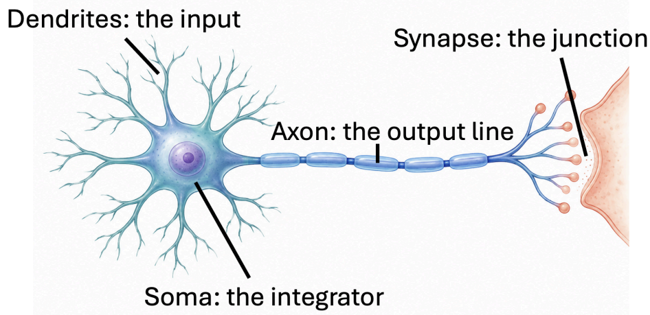
Figure 3.8 — The four roles of §3.2, and the four parts of a real cell that fill them. Signals arrive on the dendrites, are pooled in the soma, and travel out along the axon — drawn here in the segments of myelin that §3.3.5 explains — to cross at a synapse onto the next cell.
