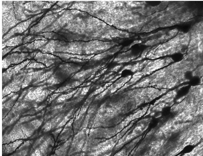
Figure 3.9 — Neurons of the dentate gyrus, stained by the Golgi method, at forty times magnification. The diagram above is a deliberate simplification, and this is what it simplifies. The branching input surface that §3.2.9's objection is about is visible here, and absent from the diagram.
