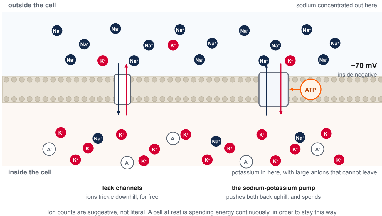
Figure 3.10 — A patch of a resting neuron's membrane. Sodium is concentrated outside and potassium inside, along with large negatively charged molecules that cannot cross at all, and the inside sits about seventy thousandths of a volt below the outside. Through leak channels the ions trickle downhill for free; the sodium–potassium pump drives them back uphill, spending a molecule of ATP each cycle. Ion counts are suggestive rather than literal.
