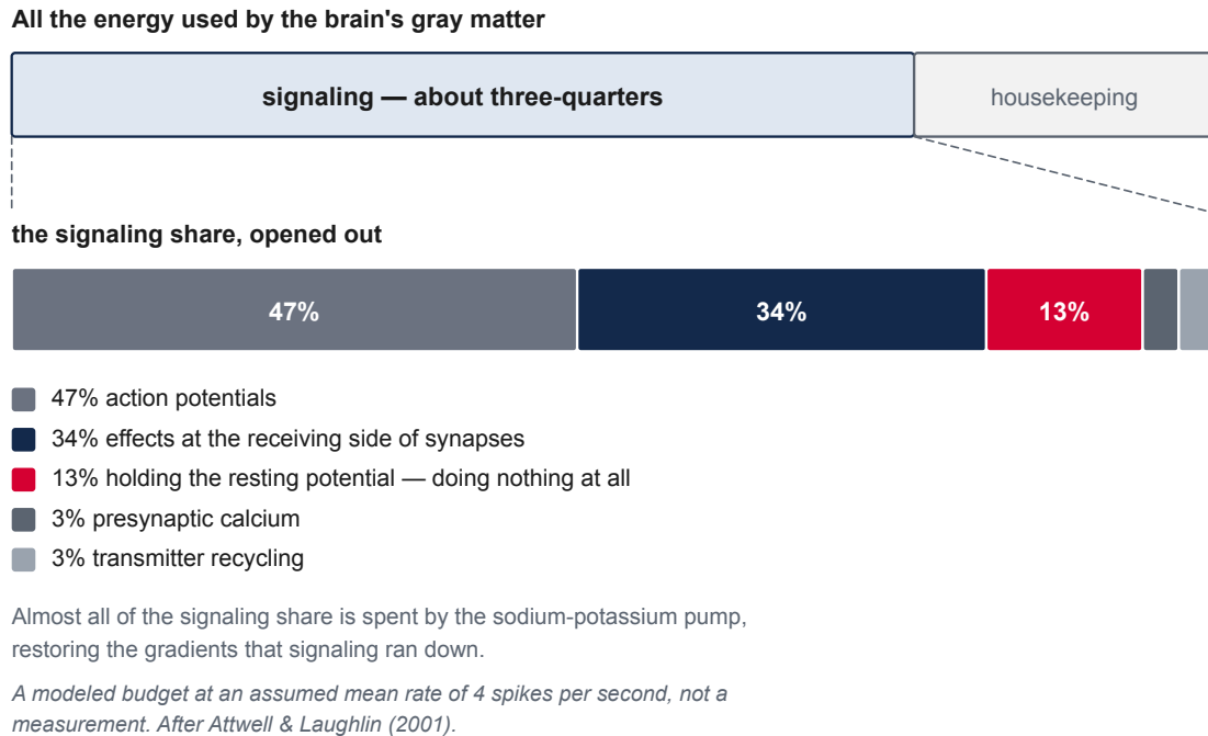
Figure 3.15 — The energy budget for the brain's gray matter, opened out in two steps. About three-quarters goes to signaling rather than to housekeeping, and almost all of that goes to the sodium–potassium pump restoring what signaling ran down. Within the signaling share, an eighth is spent by cells doing nothing at all except holding their resting potential. These are modeled figures at an assumed mean firing rate, not a measurement.
