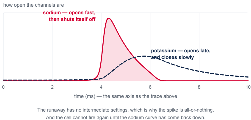
Figure 3.12 — How open the two kinds of voltage-gated channel are during the action potential above, on the same time axis. Sodium opens fast and then shuts itself off; potassium opens late and closes slowly. The rising phase is a positive feedback loop, which is why the spike has no intermediate settings, and the cell cannot fire again until the sodium curve has come back down.
