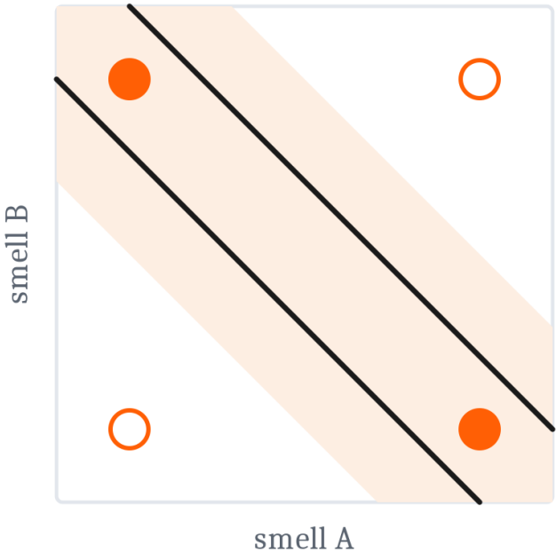
as boundaries
