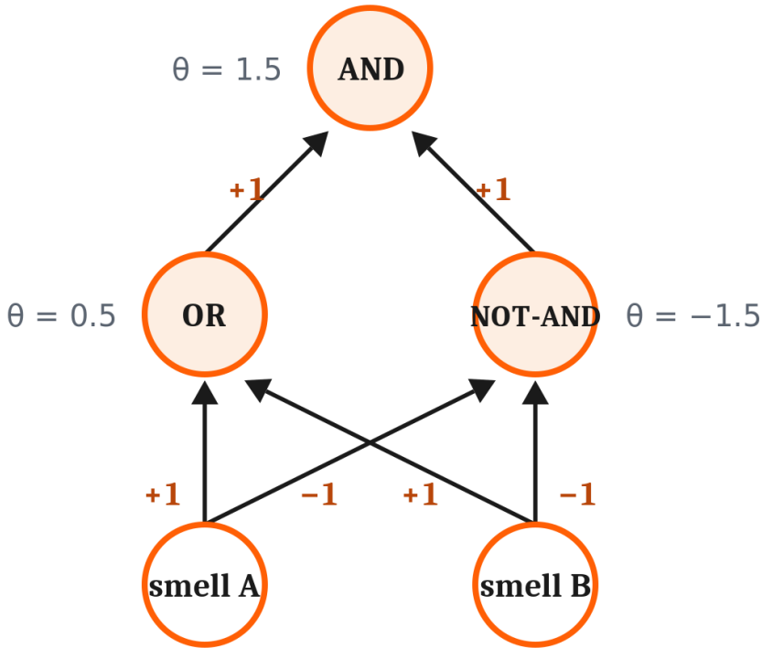
the network
