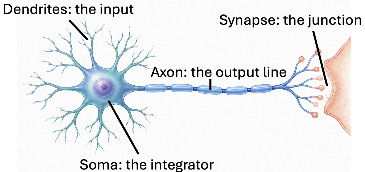
Figure 3.8 — The four roles of §3.2, and the four parts of a real cell that fill them. Signals arrive on the dendrites, are pooled in the soma, and travel out along the axon — drawn here in the segments of myelin that §3.3.5 explains — to cross at a synapse onto the next cell.
