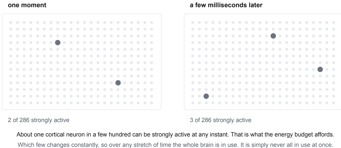
Figure 3.16 — A field of cortical neurons at two moments a few milliseconds apart. At each instant only a handful are strongly active, which is what the energy budget affords. It is a different handful each time, so over any stretch of time the whole population is used — and never all at once.
