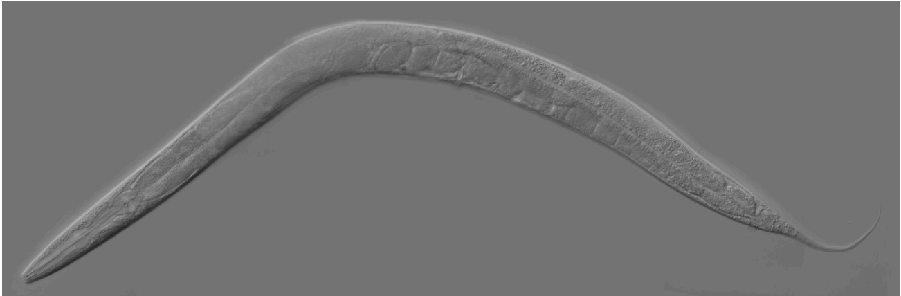
Figure 3.7 — An adult C. elegans hermaphrodite under a light microscope, about a millimeter long. Three hundred and two neurons, a complete wiring diagram, and an animal that steers toward food and reverses at an obstacle, all in a body this size.
