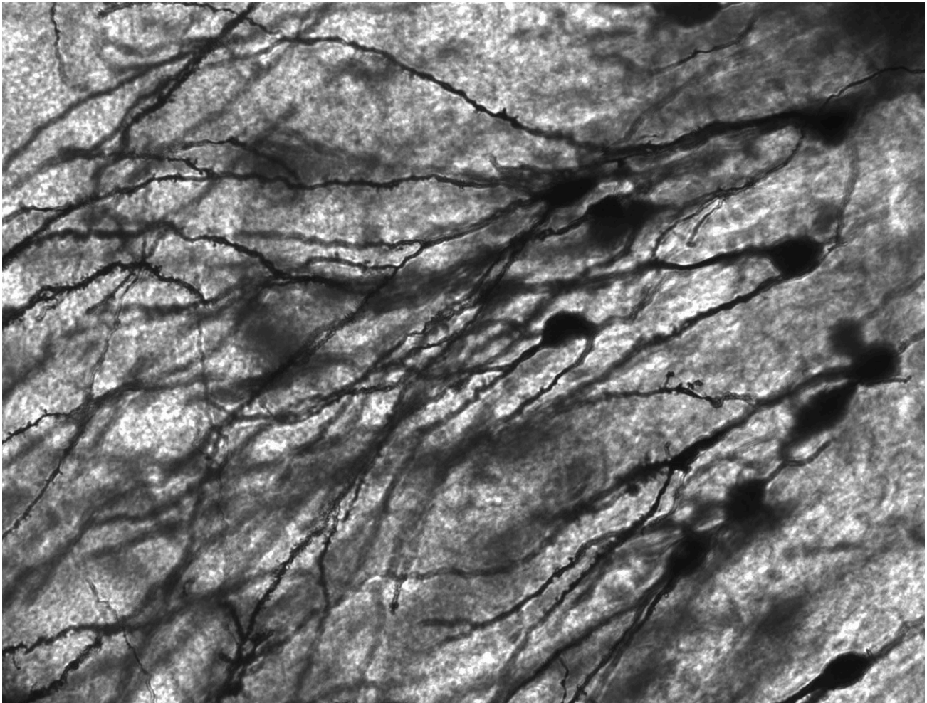
Figure 3.9 — Neurons of the dentate gyrus, stained by the Golgi method, at forty times magnification. The diagram above is a deliberate simplification, and this is what it simplifies. The branching input surface that §3.2.9's objection is about is visible here, and absent from the diagram.
