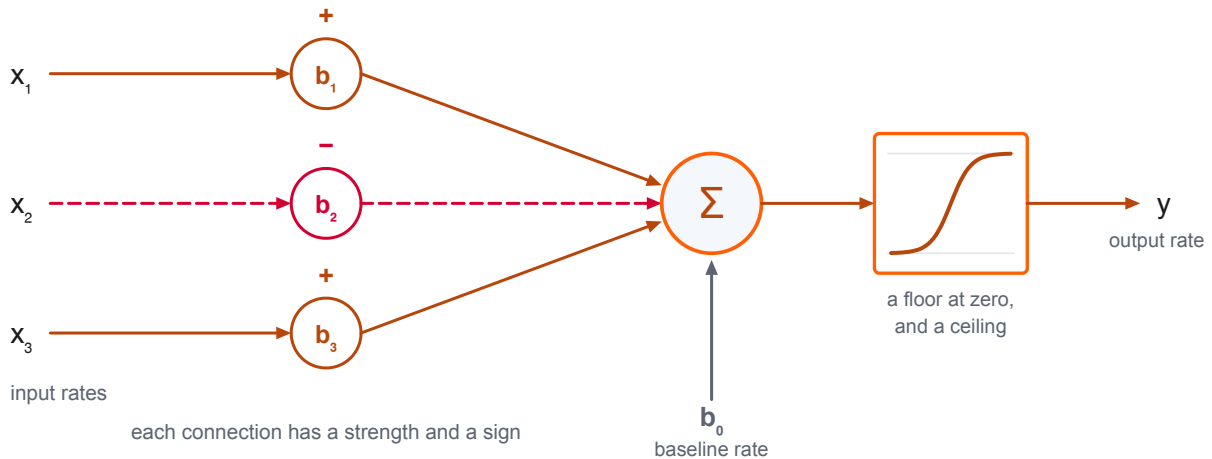
Figure 3.6 — A single unit, biological or artificial. Each input arrives with its own rate, each connection applies its own weight, the weighted inputs and the baseline are summed, and the total passes through a function that holds the output rate at or above zero.
