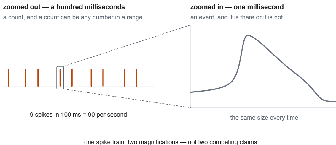
Figure 3.5 — One spike train at two magnifications. Across a hundred milliseconds there is a count, and a count can take any value in a range. Within a single millisecond there is one event, the same size as every other. The two descriptions are not competing claims about the cell; they are answers to questions asked at different time scales.
