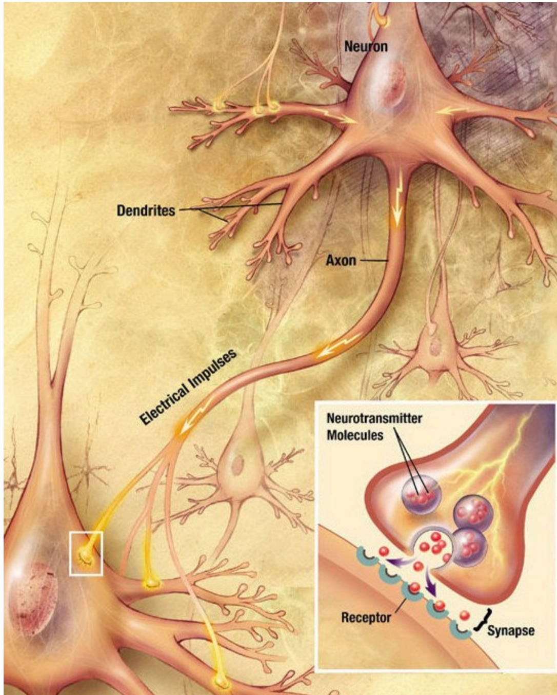
Figure 3.14 — Neurons in tissue, with one axon ending opened out. In the main panel, arrows follow the direction impulses travel, from a cell body out along its axon to the next cell. The inset enlarges a single ending: packets of neurotransmitter are released into the gap, cross it, and bind receptors on the far side.
