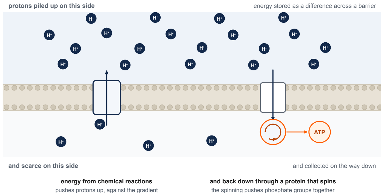
Figure 3.1 — Early life's way of making ATP, and the arrangement §3.3.2 will meet again. Energy from chemical reactions drives protons to one side of a membrane, where they pile up. They return through a protein that spins as they pass, and the spinning is the mechanical force that pushes phosphate groups together. Storing energy as a difference held across a barrier is a trick life found early and never gave up.
