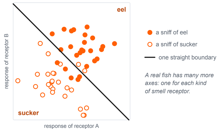
A feature space for two kinds of smell receptor
