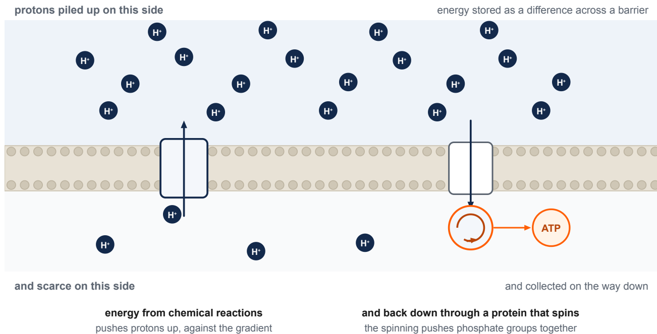
Figure 3.1 — Early life's way of making ATP, and the arrangement §3.3.2 will meet again. Energy from chemical reactions drives protons to one side of a membrane, where they pile up. They return through a protein that spins as they pass, and the spinning is the mechanical force that pushes phosphate groups together. Storing energy as a difference held across a barrier is a trick life found early and never gave up.
