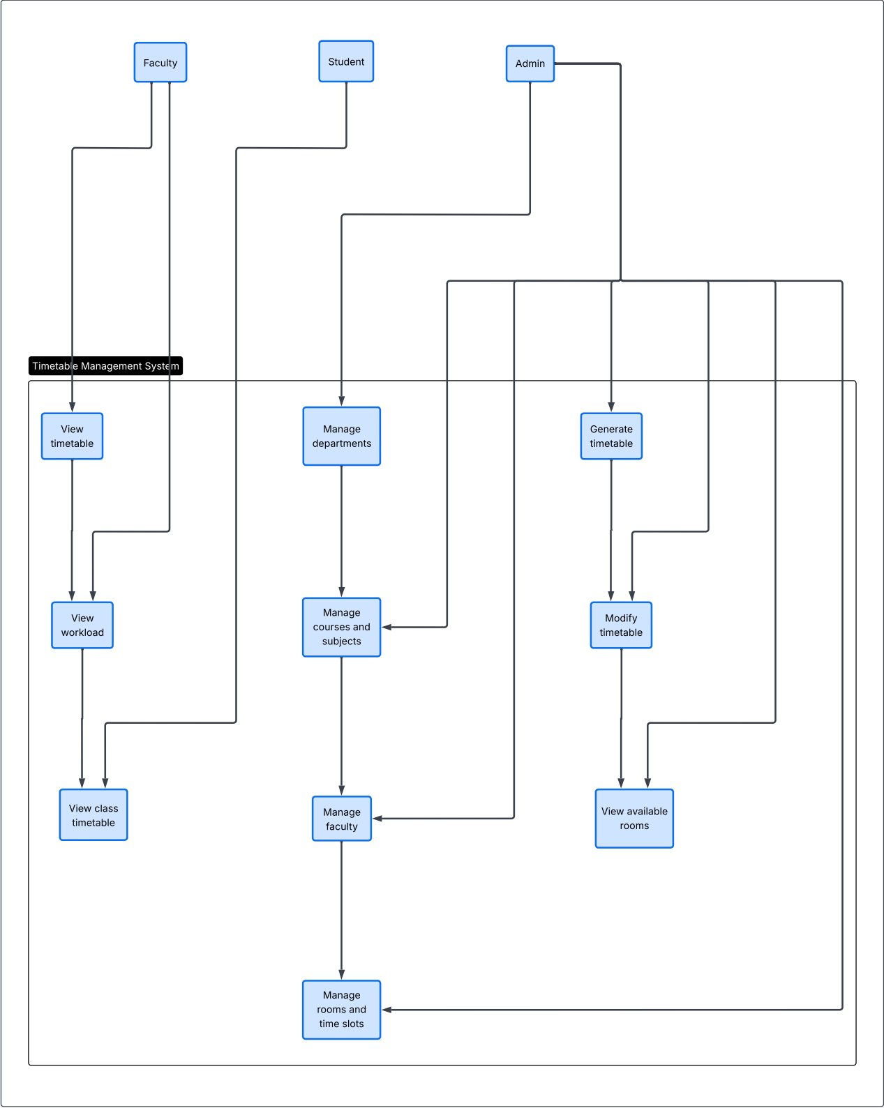
Timetable Management System Use Case Diagram
