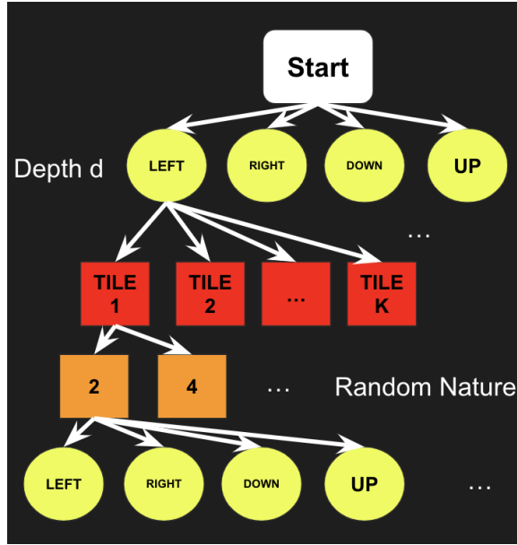
Figure 1: Game Tree
