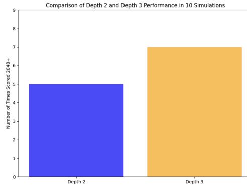
Figure 3: Using 4 Heuristics
