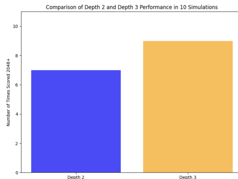
Figure 2: Using 3 Heuristics
