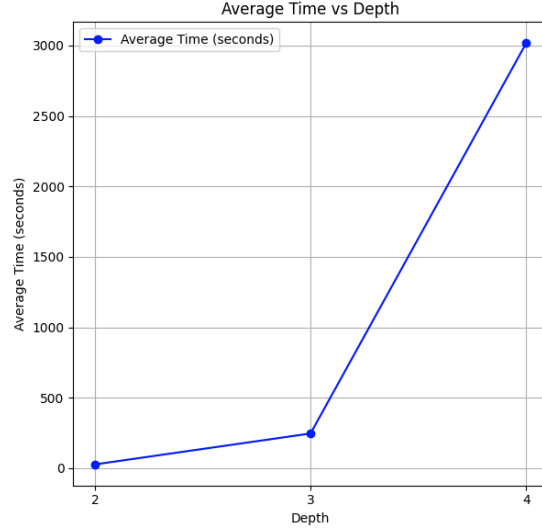
Figure 4: Comparison of Algorithm Performance and Computation Time at Different Depths
