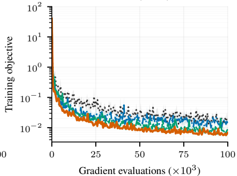
PIDM (136M)
