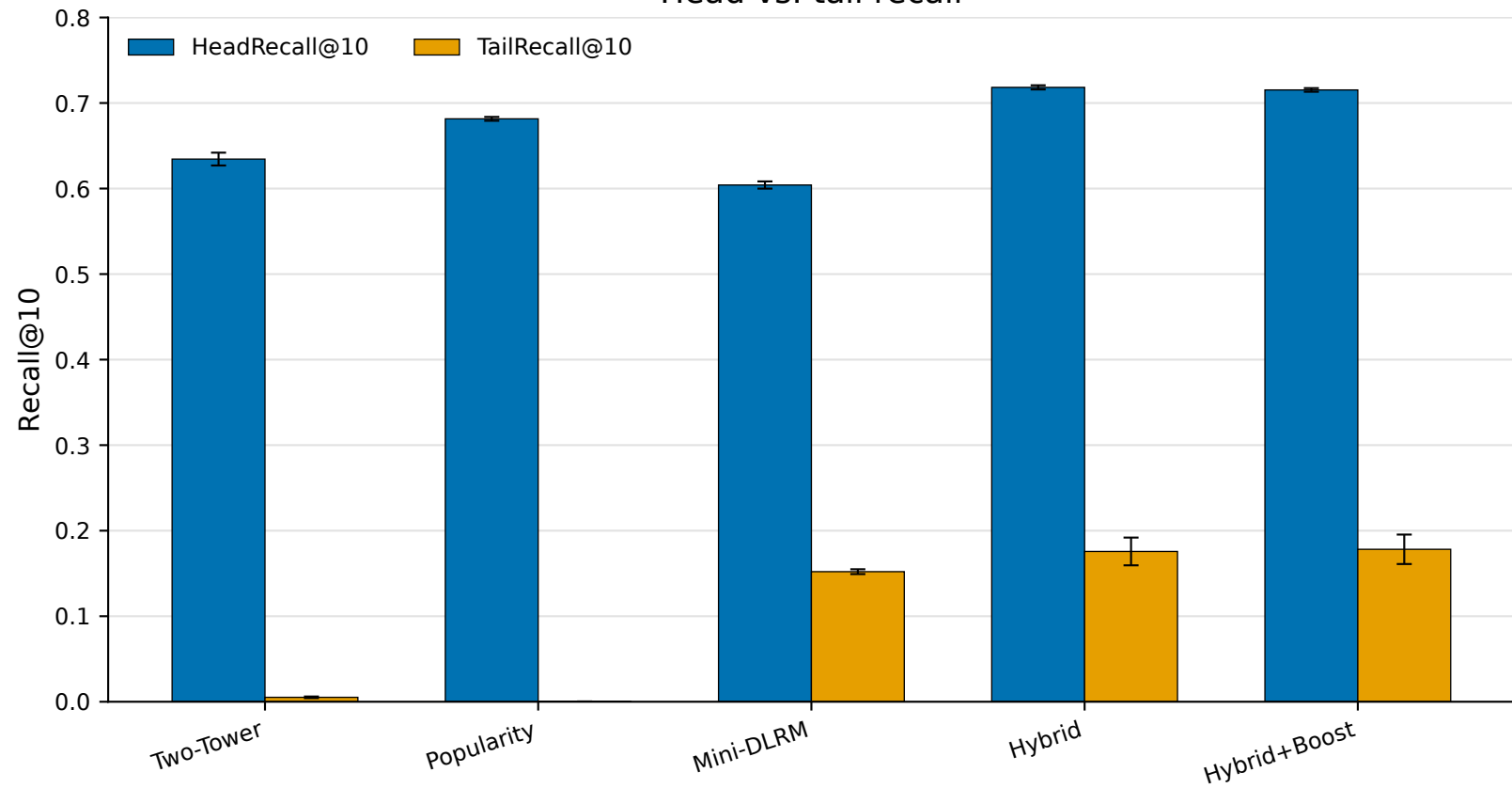
Head vs. tail recall
