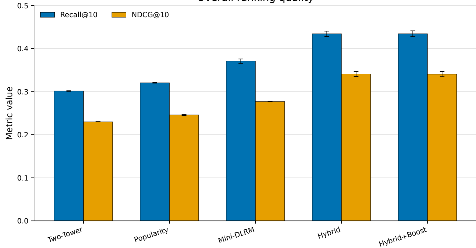
Overall ranking quality
