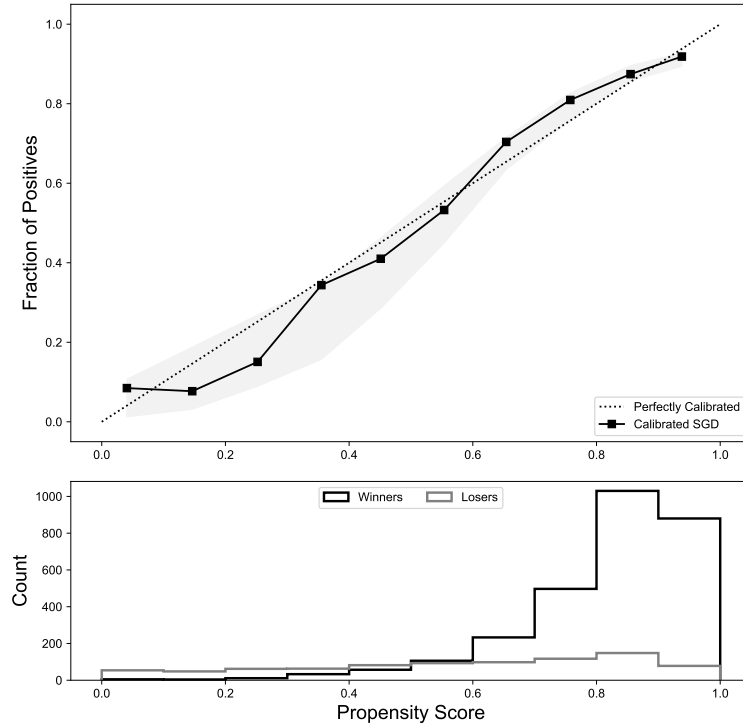
Figure 1: Text Propensity Score Calibration Plot.
