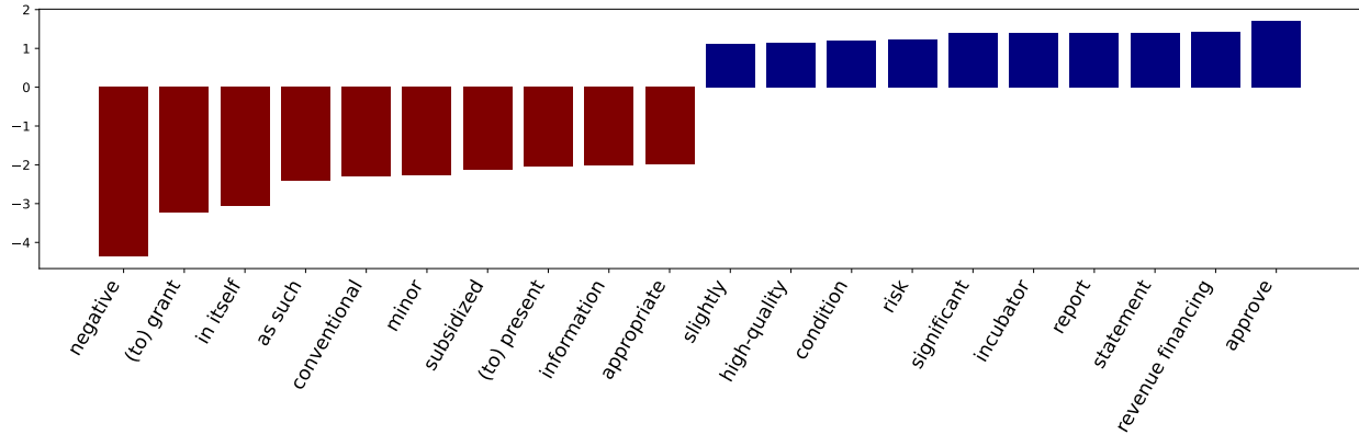
Figure H1: Predictive Words for Winning a Subsidy in the Application Texts.
