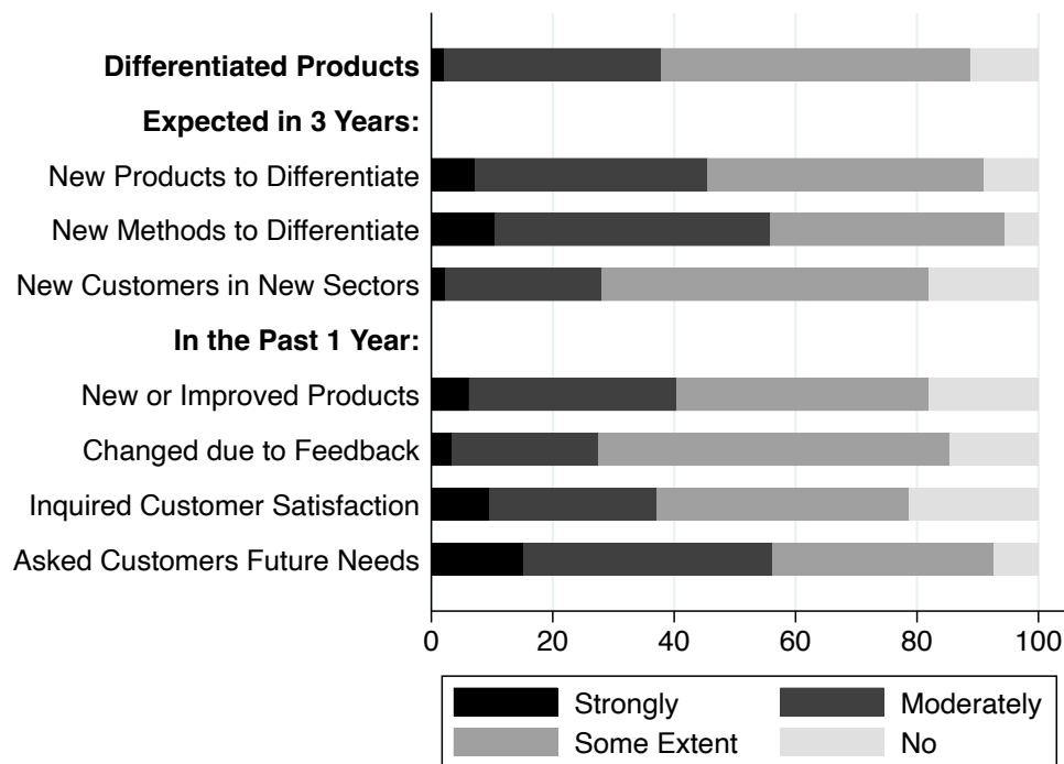
Figure A18: Etla Survey: Intentions.
