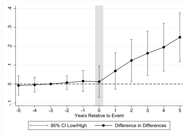
Figure 3: Employment Effects: Effect of Technology Subsidies on Employment (%).
