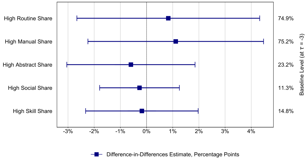
Figure A12: Skill Effects: Effect of Technology Subsidies on Task Content.
