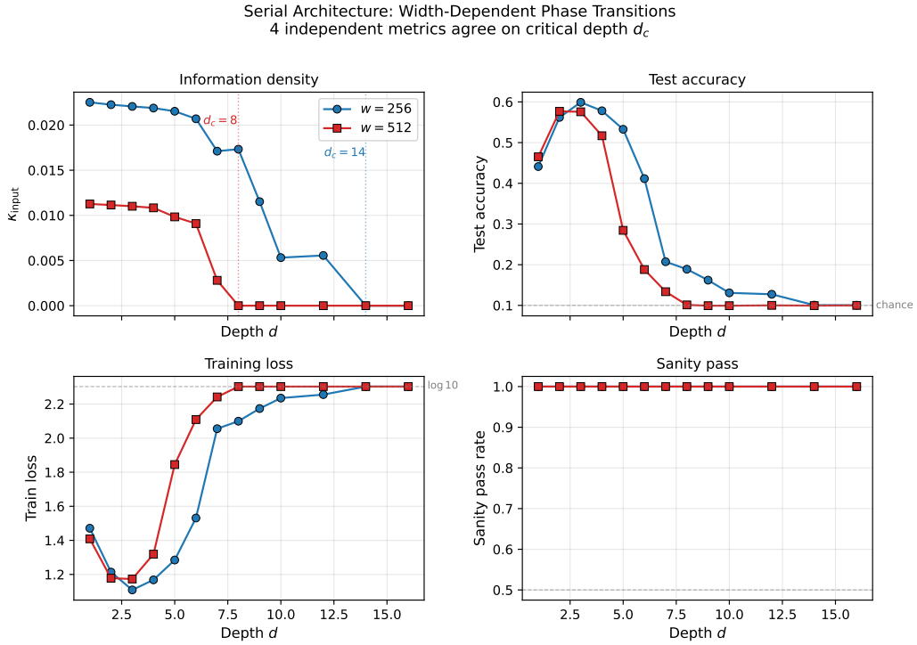
Figure 4: Figure 4. Phase transition in the Serial architecture (residual-free). Four independent metrics — information capacity \kappa_{\text{input}} , test accuracy, training loss, and sanity pass rate — agree on the critical depth d_c . For w=256 , d_c=14 ; for w=512 , d_c=8 . The simultaneous agreement across measurements with different sources of bias rules out estimator artifact.
