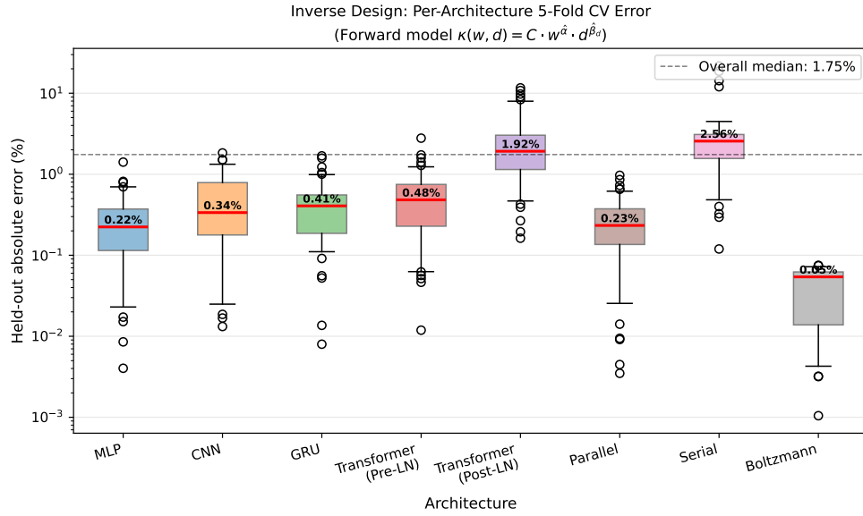
Figure 6: Figure 6. Inverse design held-out error: per-architecture 5-fold cross-validation of the two-variable forward model \kappa(w, d) = C \cdot w^{\hat{\alpha}} \cdot d^{\hat{\beta}_d} , fit separately for each architecture. Six of eight architectures achieve median error below 0.5% (best: Boltzmann at 0.05%); higher errors for Post-LN (1.92%) and Serial (2.56%) reflect their depth-sensitivity and phase-transition behaviour (see Section 7). The pooled global model (single \kappa(w, d) for all architectures) gives 1.75% overall median.
