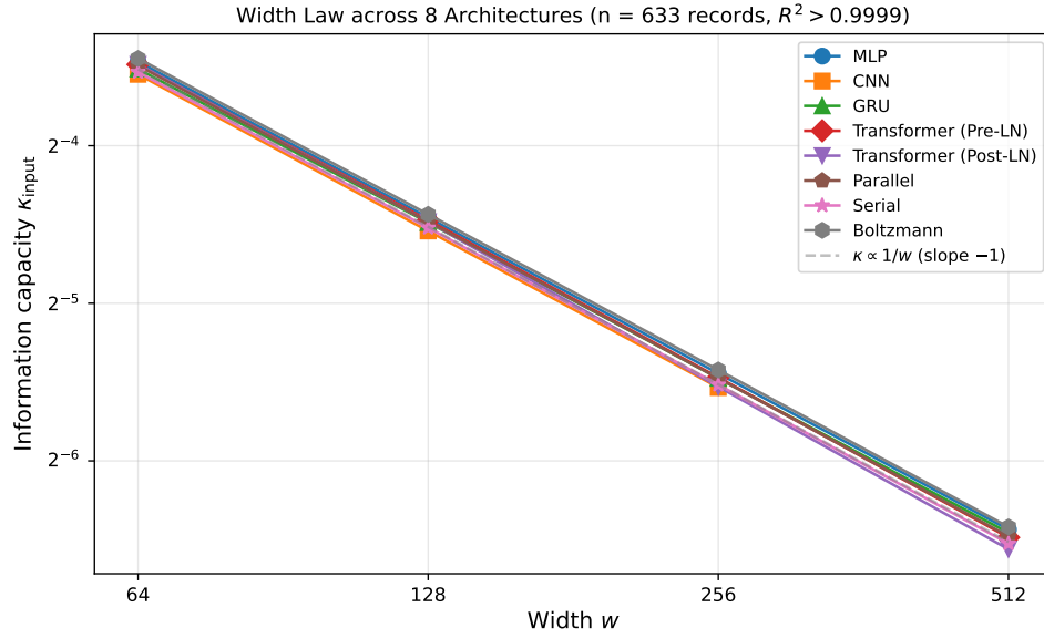
Figure 3: Figure 3. Width law across eight neural architectures. The per-record information capacity \kappa_{\text{input}} scales as \kappa \propto 1/w across all architectures ( n = 633 records, R^2 > 0.9999 ). Lines connect width-averaged means; the dashed reference line shows slope -1 .
