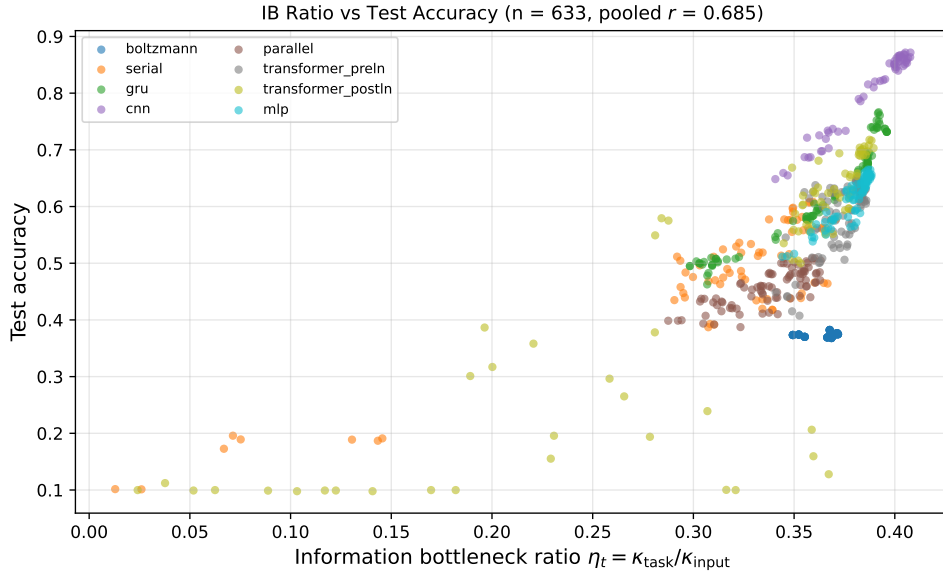
Figure 5: Figure 5. The information bottleneck ratio \eta_t = \kappa_{\text{task}}/\kappa_{\text{input}} correlates with test accuracy across n = 633 records (pooled r = 0.685 ). The d_z denominator cancels exactly between numerator and denominator, so this signal is not an artifact of per-dimension normalization. Per-architecture correlations are r > 0.65 in 7 of 8 architectures; the exception is Boltzmann ( r = +0.17 ), consistent with RBMs not being optimized for classification.
