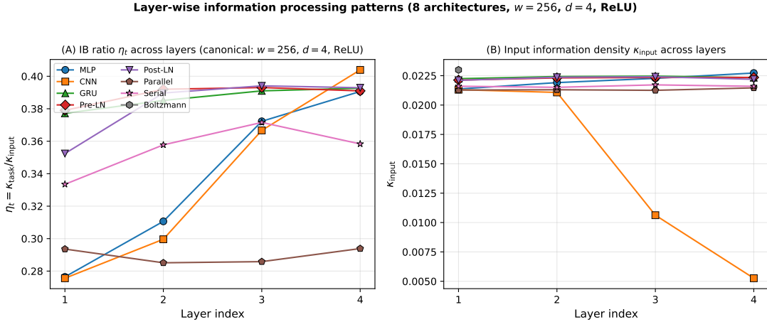
Figure 7: Figure 7. Layer-wise information processing patterns at the canonical configuration ( w=256 , d=4 , ReLU). Left: information bottleneck ratio \eta_t across layers. MLP and CNN show monotonic increases (+41% and +47% from L1 to L4 respectively), consistent with deeper layers carrying more task-aligned information. Pre-LN, GRU, and Parallel show flat profiles. Post-LN shows a smaller increase (+12%). Right: \kappa_{\text{input}} across layers; the visible drop in CNN at L3-L4 is dimension-dependent and explained quantitatively in Section 11.3.
