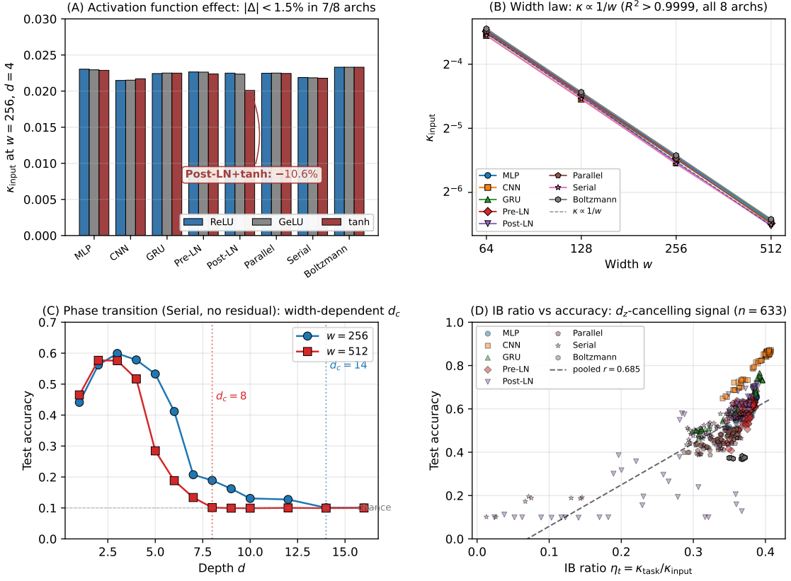
Figure 1: Figure 1. Visual summary of the four observations. (A) Activation functions are not a major determinant of \kappa_{\text{input}} (7 of 8 architectures within |\Delta| < 1.5\% of ReLU; the single exception is Post-LN with tanh). This negative result motivates examination of structural variables (Section 3). (B) Width is the dominant determinant: \kappa \propto 1/w with R^2 > 0.9999 across all eight architectures (Section 4). (C) Architectures without residual connections undergo width-dependent phase transitions; the Serial architecture collapses at d_c=14 for w=256 and d_c=8 for w=512 (Section 7). (D) The information-bottleneck ratio \eta_t = \kappa_{\text{task}}/\kappa_{\text{input}} , in which the per-dimension normalization d_z cancels exactly, correlates with test accuracy at pooled r = 0.685 ( n = 633 ); this signal is therefore not an artifact of d_z -normalization (Section 9).
