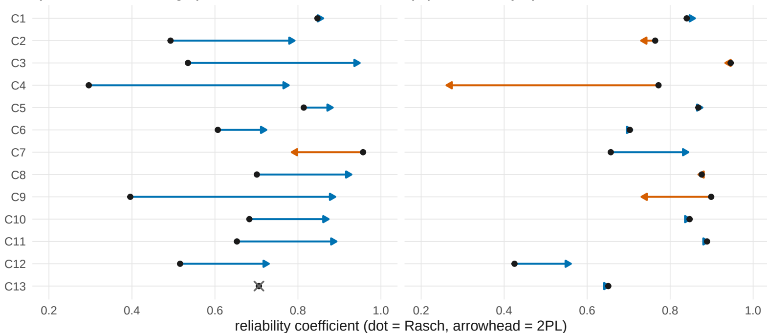
Gaussian-fit mirt marginal_rxx (information-ratio catalogue)
