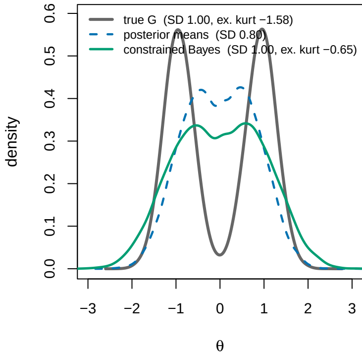
What constrained Bayes fixes, and does not
