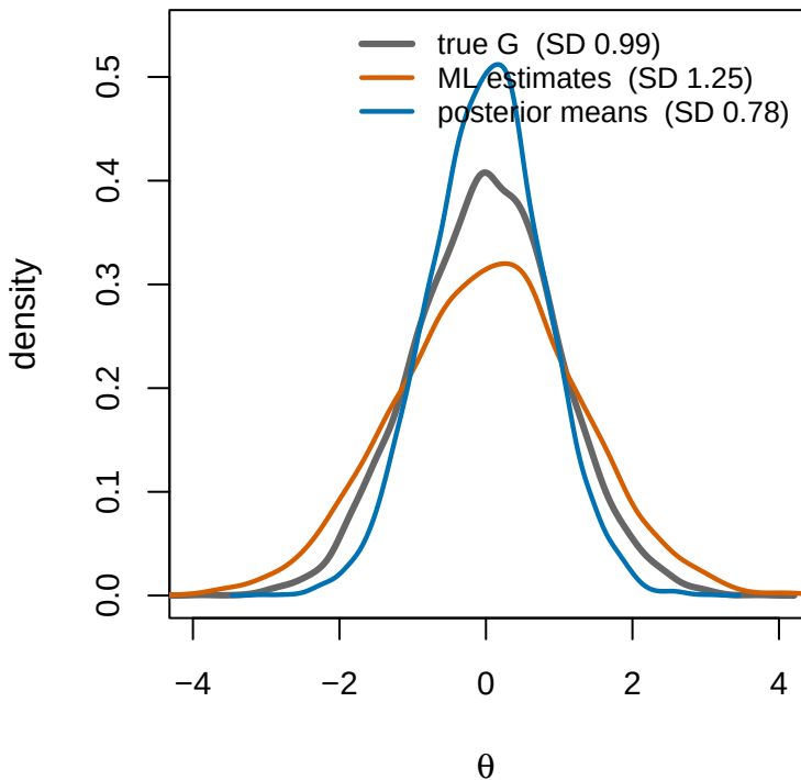
One truth, two wrong histograms
