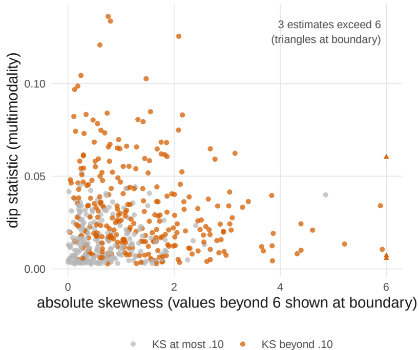
Skew is the common departure; multimodality is rare
