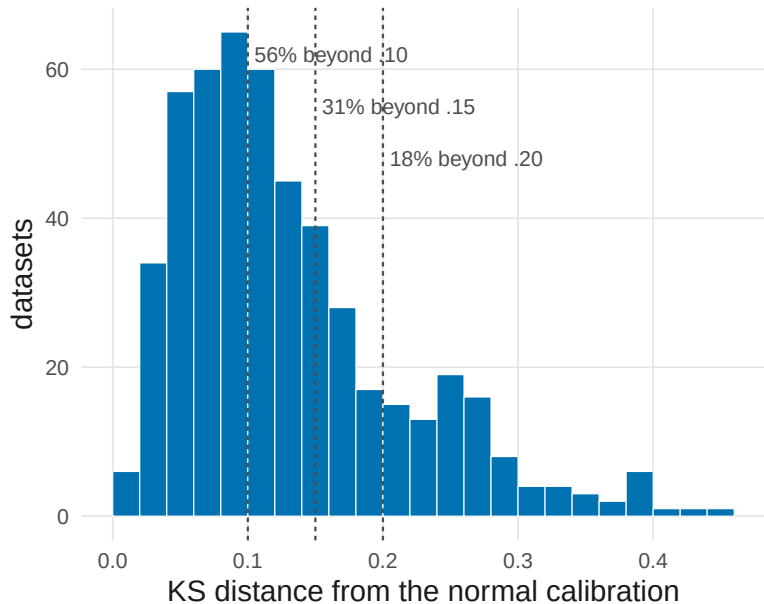
How far the fitted latent distribution sits from normal
